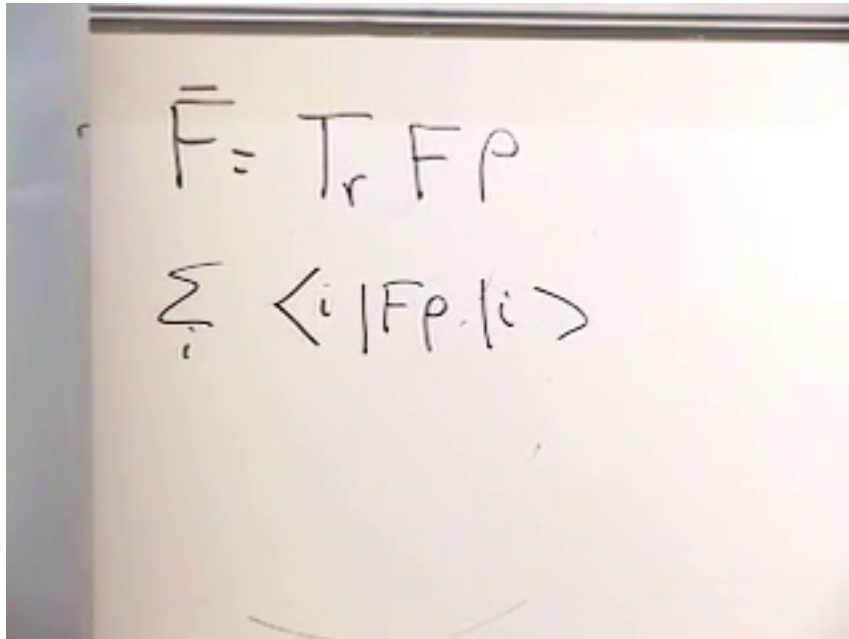
Figure 7.10: The trace expectation value \langle F \rangle = \text{Tr}(F\rho) .
