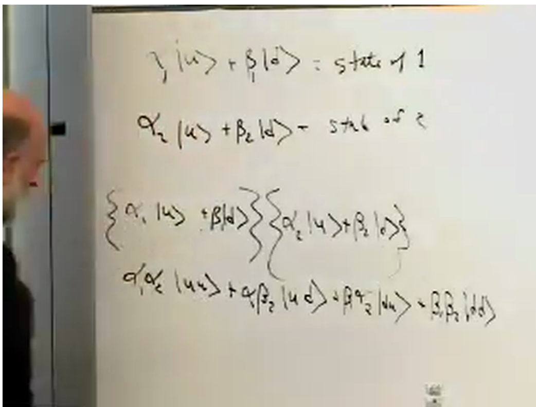
Figure 4.8: Multiplying two one-spin states produces a restricted four-term product state.
