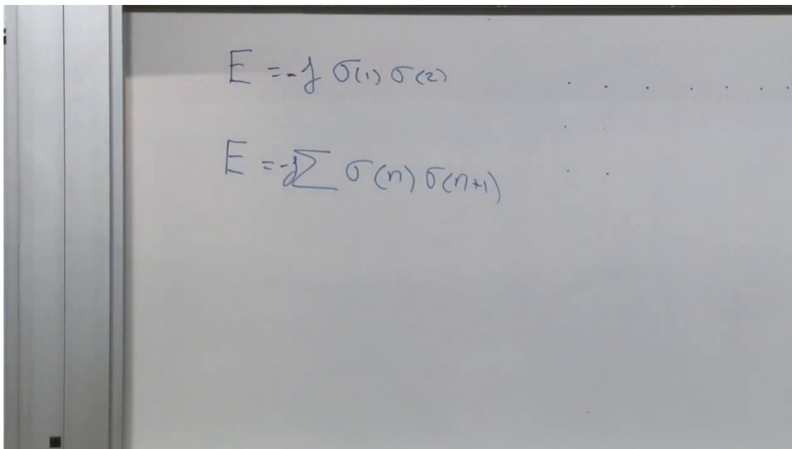
Figure 1.9: The local pair energy extended to the nearest-neighbor chain Hamiltonian.
