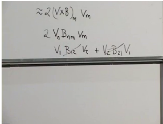
Figure 6.6: The paired terms in v_n B_{nm} v_m cancel because the magnetic tensor changes sign when its indices are interchanged.
