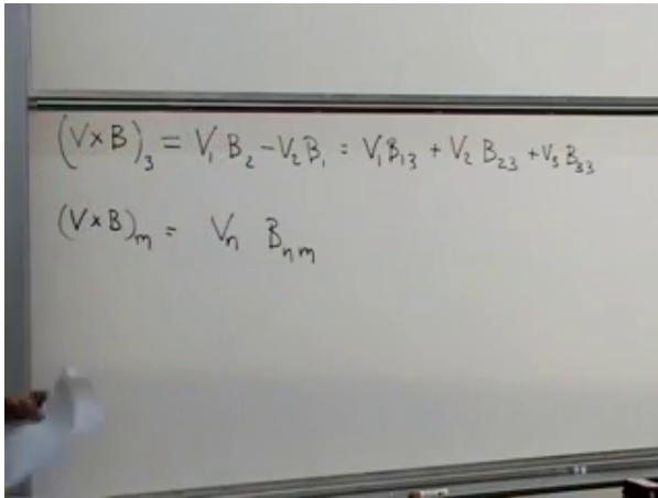
Figure 6.5: The third component of \mathbf{v} \times \mathbf{B} and its general expression as a contraction with B_{nm} .
