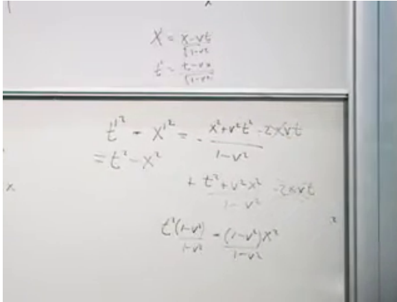
Figure 3.4: The board derivation of t'^2 - x'^2 = t^2 - x^2 .
