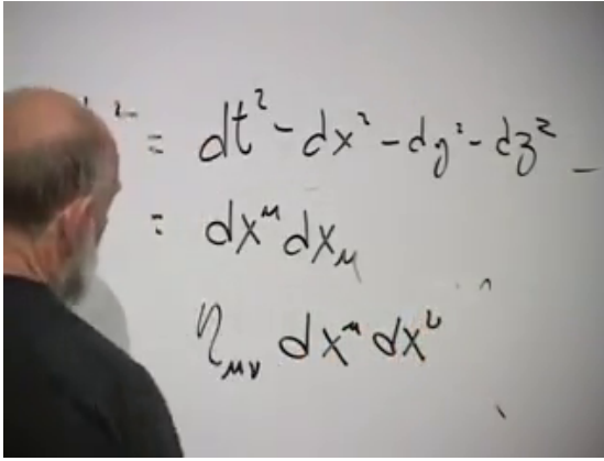
Figure 7.3: The Minkowski interval written successively in component, contracted-index, and metric-tensor notation.
