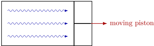
Figure 8.22: Clean reconstruction of the radiation-piston analogy.
