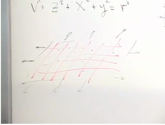
Figure 8.5: A coordinate mesh carried along by an expanding spatial sheet. Source frame at 00:22:20.
