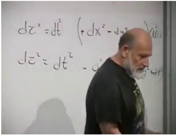
Figure 7.12: The spatially flat cosmological metric as completed on the board, with the common factor a^2(t) multiplying all three spatial directions.
