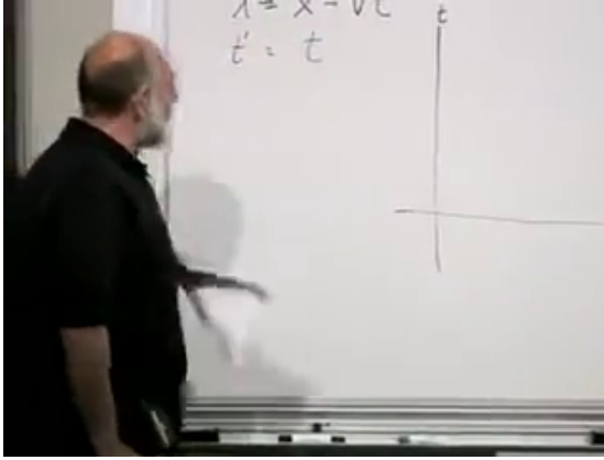
Figure 3.1: The Galilean transformation and the initial t - x grid. The moving origin will trace x = vt , while the two frames retain common constant-time lines.
