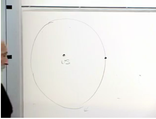
Figure 8.8: The shell-theorem construction: us at the center and a test galaxy on the boundary of a large homogeneous sphere. Source frame at 00:41:10.
