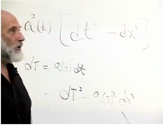
Figure 8.23: The time redefinition dT = A(t)dt that converts conformal time to cosmic time. Source frame at 01:51:05.
