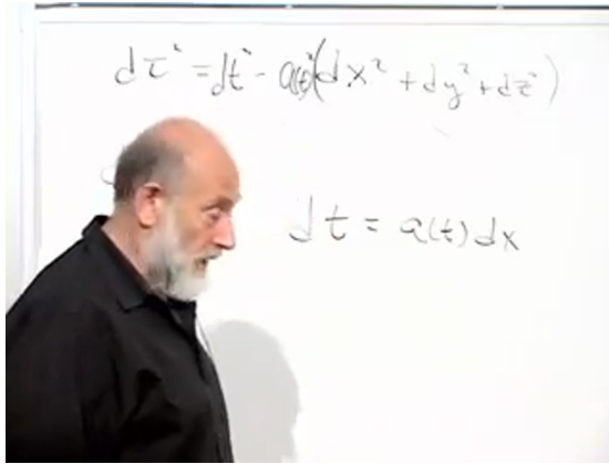
Figure 8.7: The null condition and dt = a(t)dx for radial light propagation. Source frame at 00:30:54.
