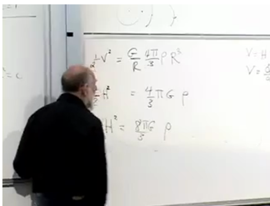
Figure 8.12: The cancellation of the radius and the resulting flat Friedmann relation on the board. Source frame at 00:57:30.
