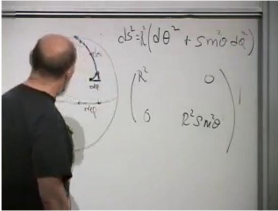
Figure 7.8: The sphere, its angular line element, and the corresponding metric matrix. The \sin^2 \theta factor records the shrinking circles of latitude.
