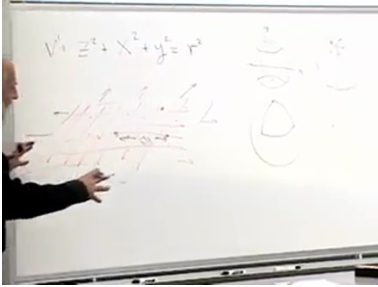
Figure 8.4: Positive, zero, and negative curvature sketched through their characteristic triangle shapes. Source frame at 00:37:30.
