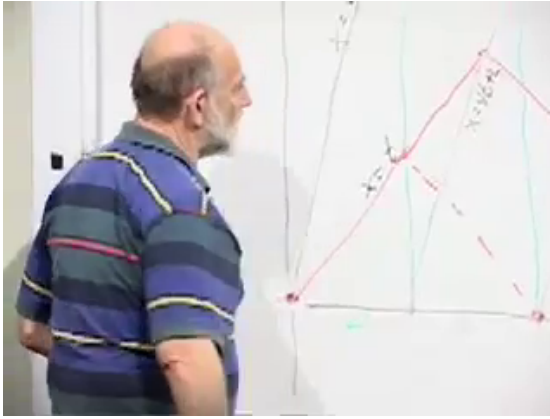
Figure 1.4: The forward light ray x = t meeting the middle moving worldline.
