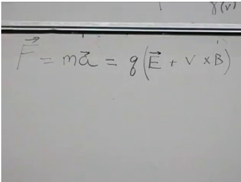
Figure 5.6: The pre-relativistic form of the Lorentz force law that motivates combining \mathbf{E} and \mathbf{B} .
