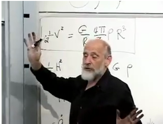
Figure 8.20: The boxed Newtonian energy equation above its Friedmann form during the energy-conservation discussion. Source frame at 01:44:42.440.
