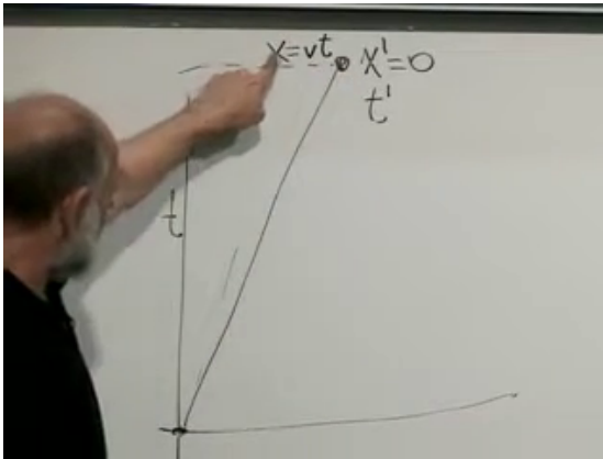
Figure 3.6: The moving origin: x = vt , x' = 0 , and the t' -axis are three descriptions of the same worldline.
