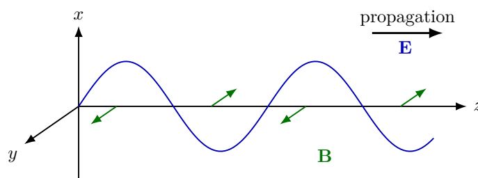
Figure 1.9: The fields \mathbf{E} and \mathbf{B} are perpendicular to each other and to the direction of propagation.
