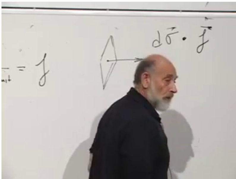
Figure 1.10: An oriented area element and the flux factor d\boldsymbol{\sigma} \cdot \mathbf{J} .
