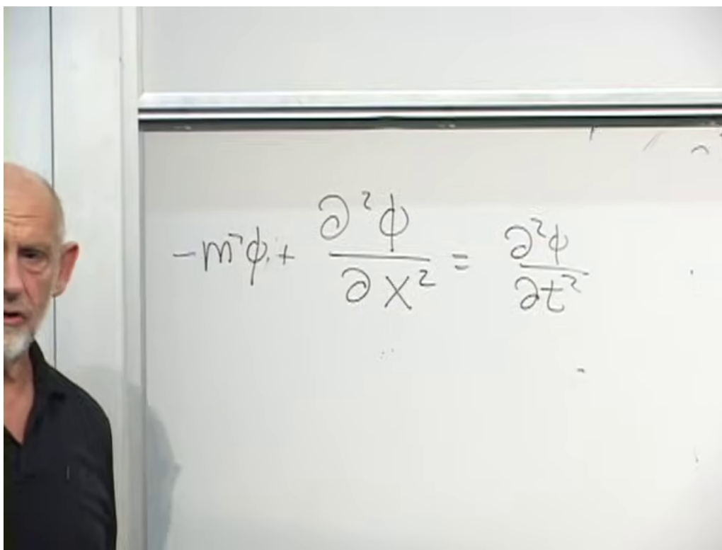
Figure 1.12: The Klein–Gordon equation used to expose the instability behind negative mass squared.
