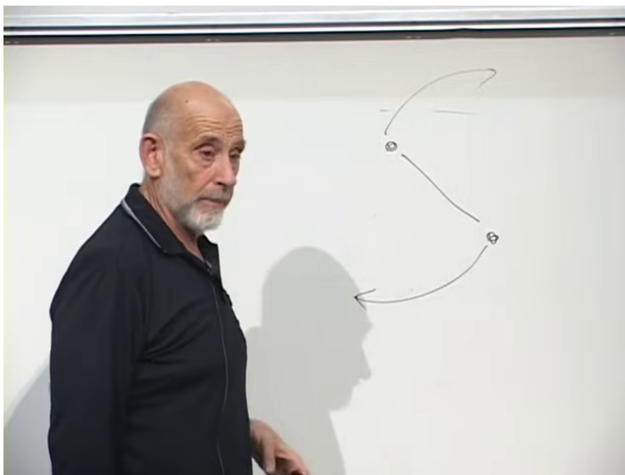
Figure 1.15: A rotating open string sketched about its center-of-mass point.
