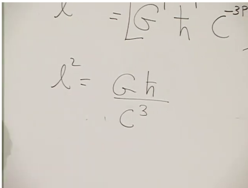
Figure 1.5: The completed dimensional argument for the Planck area and length.
