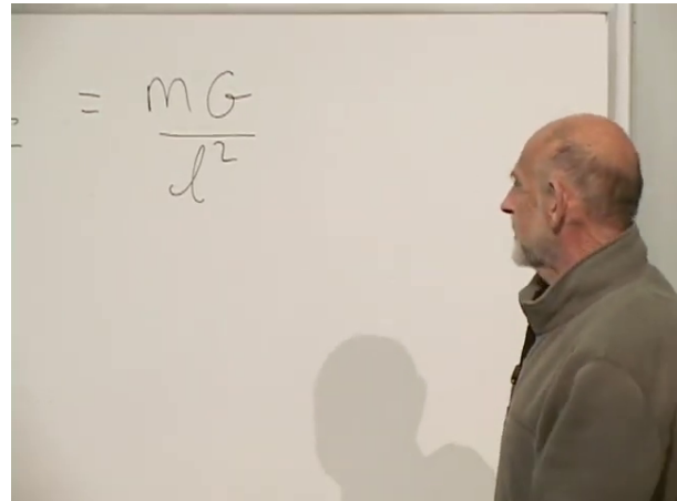
(b) Units of G from Newtonian acceleration.
