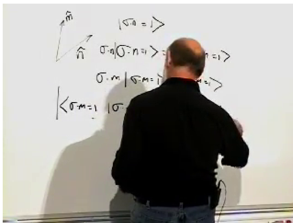
Figure 4.4: The overlap between the prepared n -state and the tested m -state is the probability amplitude.
