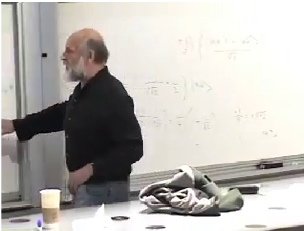
Figure 5.10: The completed board calculation displays the smaller Bell left-hand side and the larger right-hand side.
