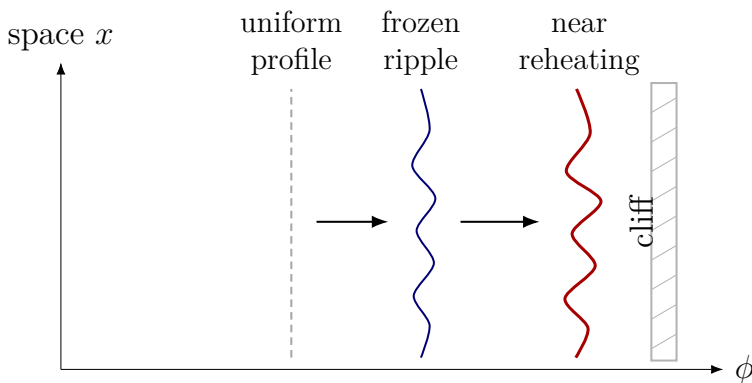
Figure 10.7: Clean reconstruction of the space-versus-field picture. The mean field moves toward the cliff while a frozen spatial ripple persists, so different positions reach the end of inflation at slightly different times.
