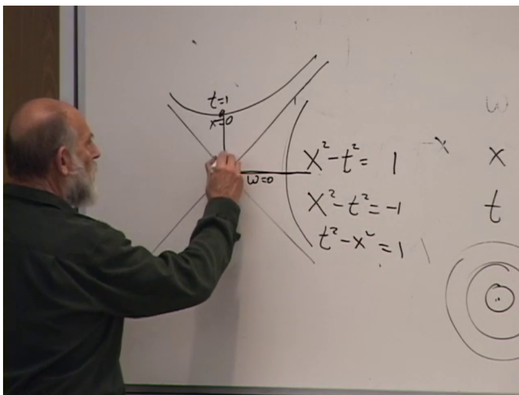
Figure 1.7: Constant- R_{\text{aux}} hyperbolae on opposite sides of the Rindler horizon. The sign change turns fixed-coordinate curves from timelike to spacelike without changing the underlying flat geometry.
