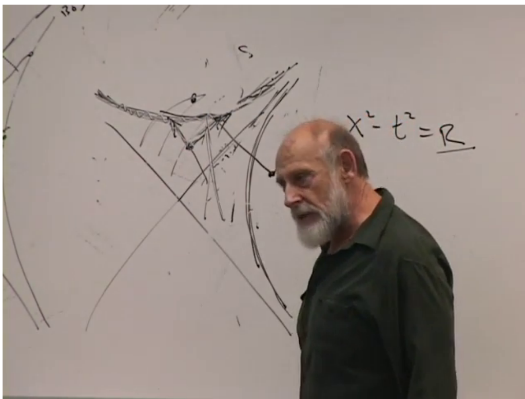
Figure 1.13: The maximally extended local picture: the horizon is a regular null boundary, whereas r = 0 is a spacelike future singularity reached by every future-directed interior worldline.
