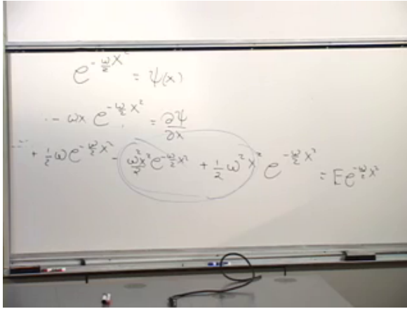
Figure 10.11: The Gaussian eigenfunction calculation leaves the zero-point energy after the quadratic terms cancel.
