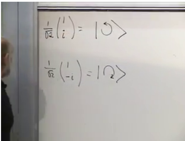
Figure 1.9: The two normalized complex vectors that form the circular polarization basis.
