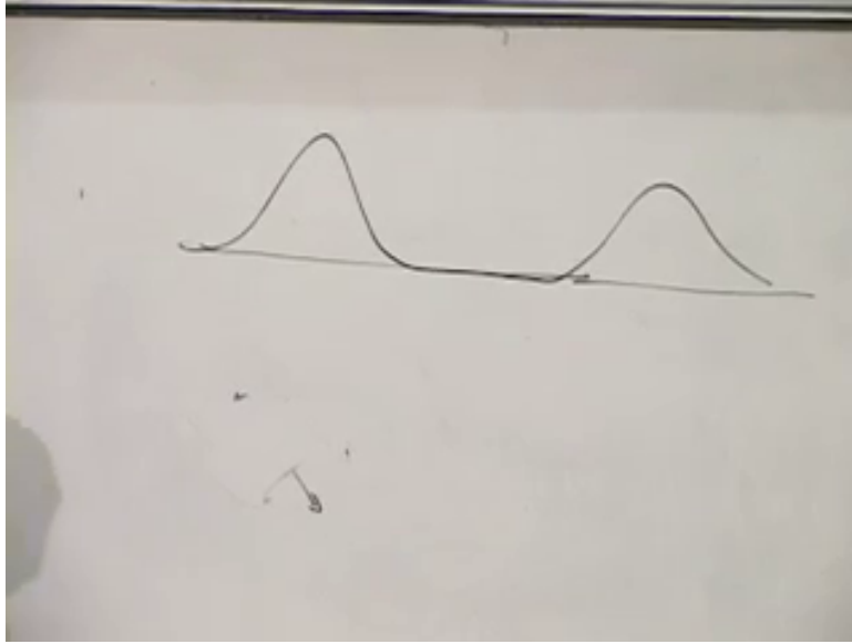
Figure 1.13: A symmetric two-lobe profile can have average position zero even though its central probability is very small.
