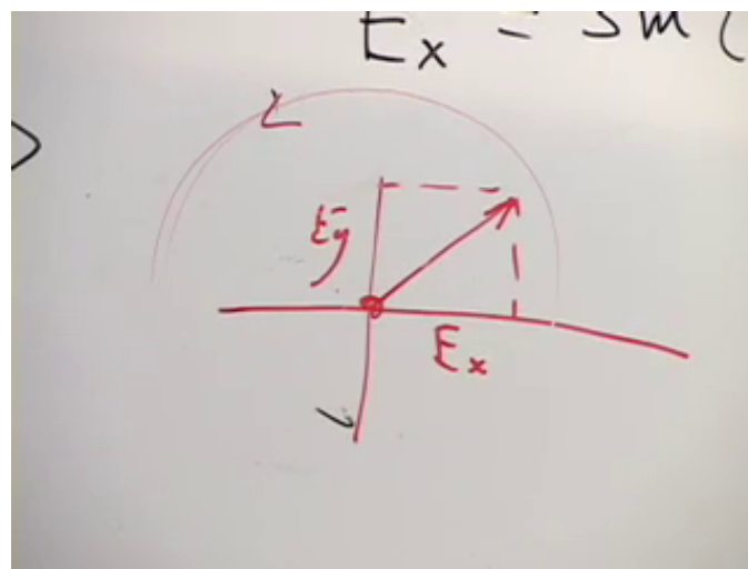
Figure 1.11: At fixed z , the two quadratures make the electric-field vector rotate.
