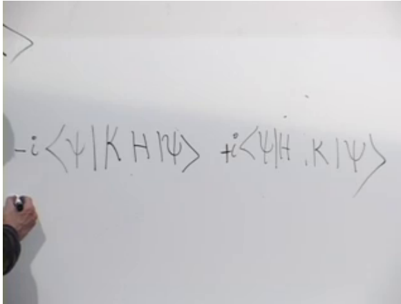
Figure 8.14: Differentiating the expectation-value sandwich produces the two operator orderings \hat{H}\hat{K} and \hat{K}\hat{H} .
