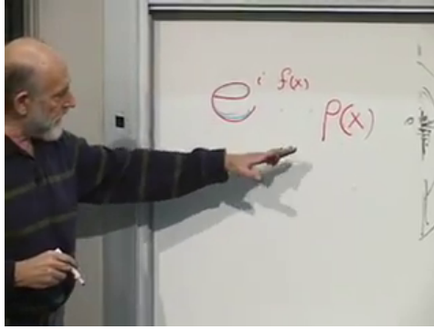
Figure 4.13: A rapidly varying phase multiplied by a smooth envelope gives a smooth one-aperture probability density.
