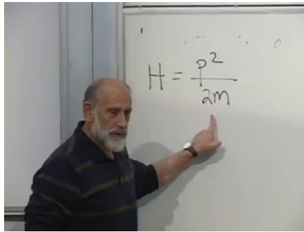
Figure 9.4: The nonrelativistic free-particle Hamiltonian chosen as an even function of momentum.
