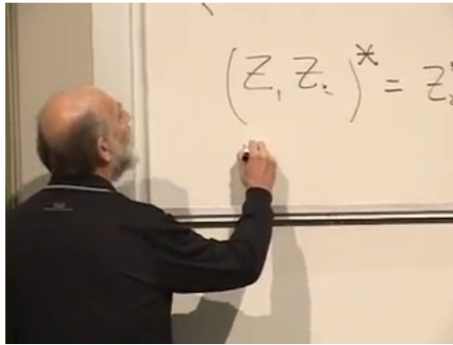
Figure 2.2: Complex conjugation of a product on the board. The corrected relation is given cleanly in Eqs. (2.4) and (2.5).
