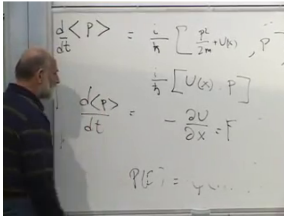
Figure 9.22: The second Ehrenfest equation: the mean momentum changes by the expectation value of the force.
