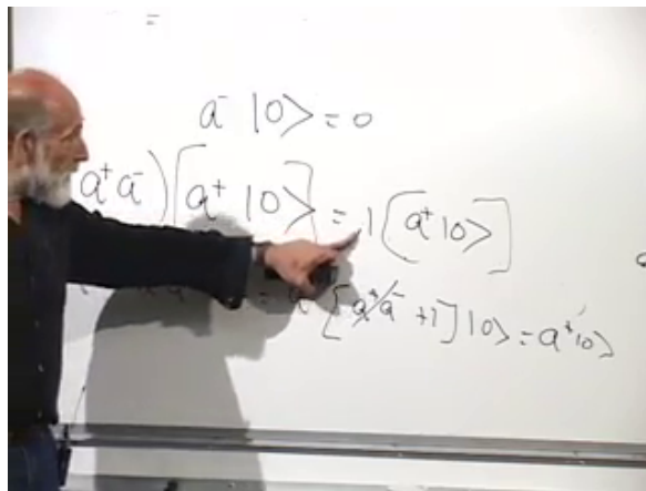
Figure 10.18: Commuting the number operator through \hat{a}^\dagger raises its eigenvalue by one.
