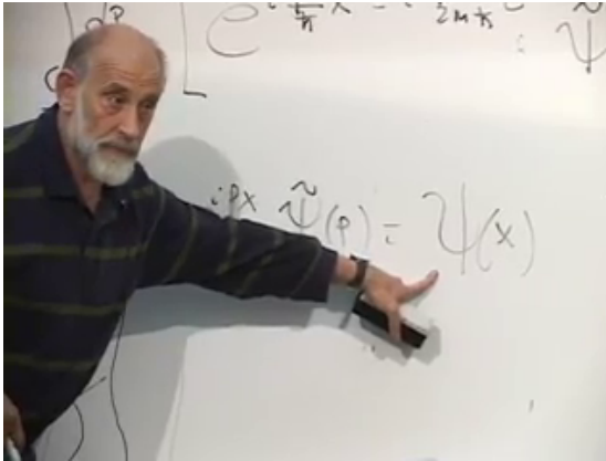
Figure 9.12: Setting t = 0 identifies the momentum superposition with the initial position-space wave function.
