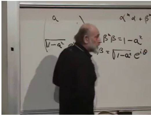
Figure 7.6: Normalization and phase fixing reduce two complex amplitudes to two physical real parameters.
