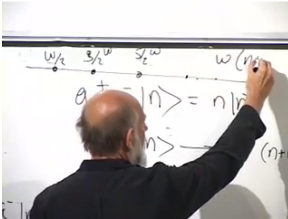
Figure 10.21: The equally spaced oscillator spectrum beginning at the zero-point energy.
