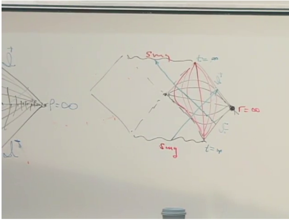
Figure 4.7: The completed eternal Schwarzschild Penrose diagram, with singularities, horizons, null trajectories, and one asymptotic boundary marked on the board.
