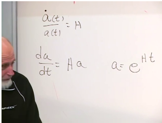
Figure 7.13: The constant- H equations and their exponential solution on the board.
