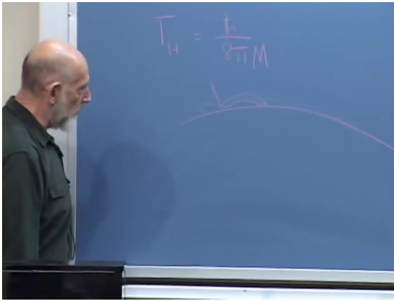
Figure 9.2: The narrow escape cone for near-horizon radiation. Most locally emitted quanta return to the horizon.
