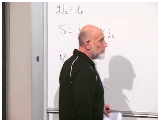
Figure 7.4: The string-side column assembled before the comparison: \ell_p \sim g_s \ell_s , S_{\text{str}} \sim L/\ell_s \sim M \ell_s , and M \sim L/\ell_s^2 .
