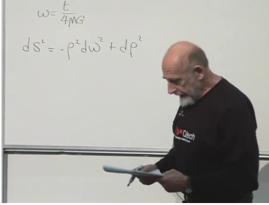
Figure 4.1: The near-horizon metric and the rescaled Schwarzschild time.
