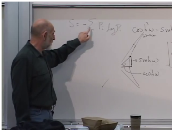
Figure 3.7: The closing board formula S = -\sum_i p_i \log p_i , written while distinguishing a probability distribution from the single entropy value computed from it.
