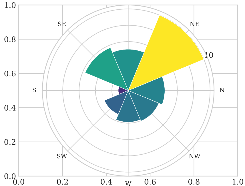
Directional intensity
