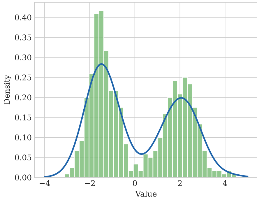
Bimodal distribution
