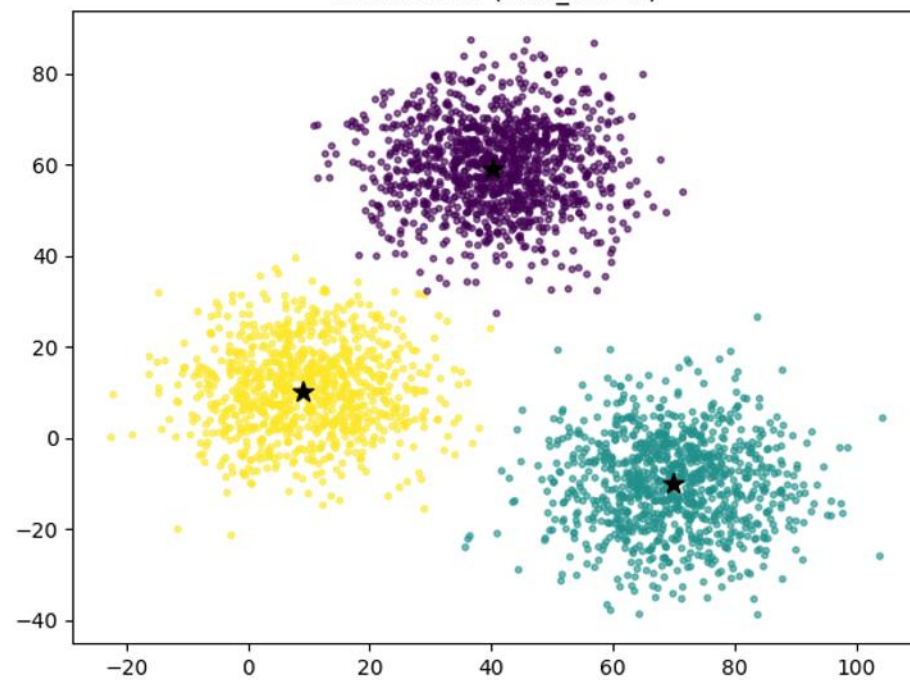
K-means++ (max_iter=1)
