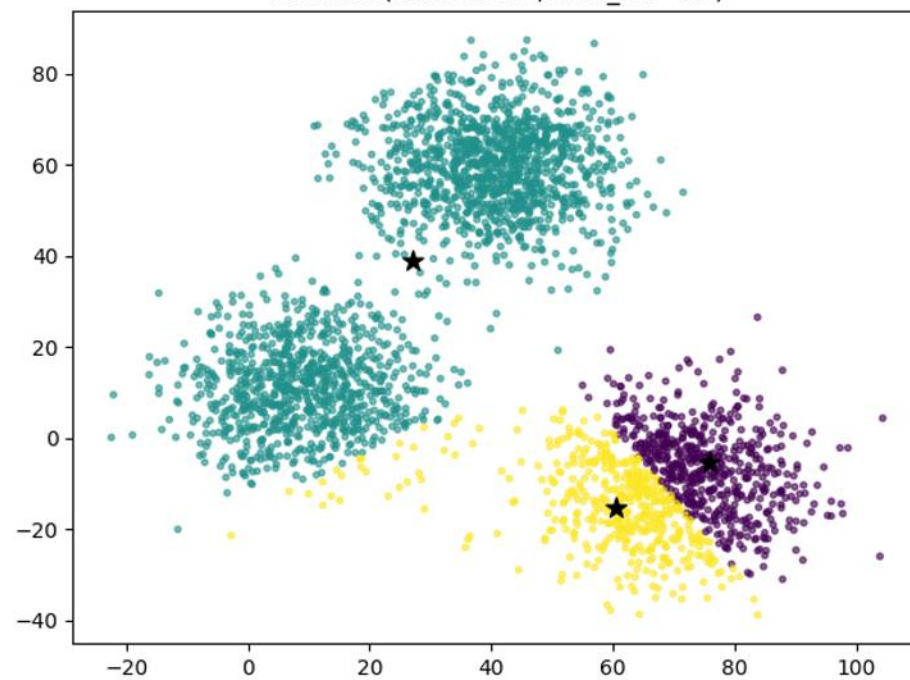
K-means (random init, max_iter=10)
