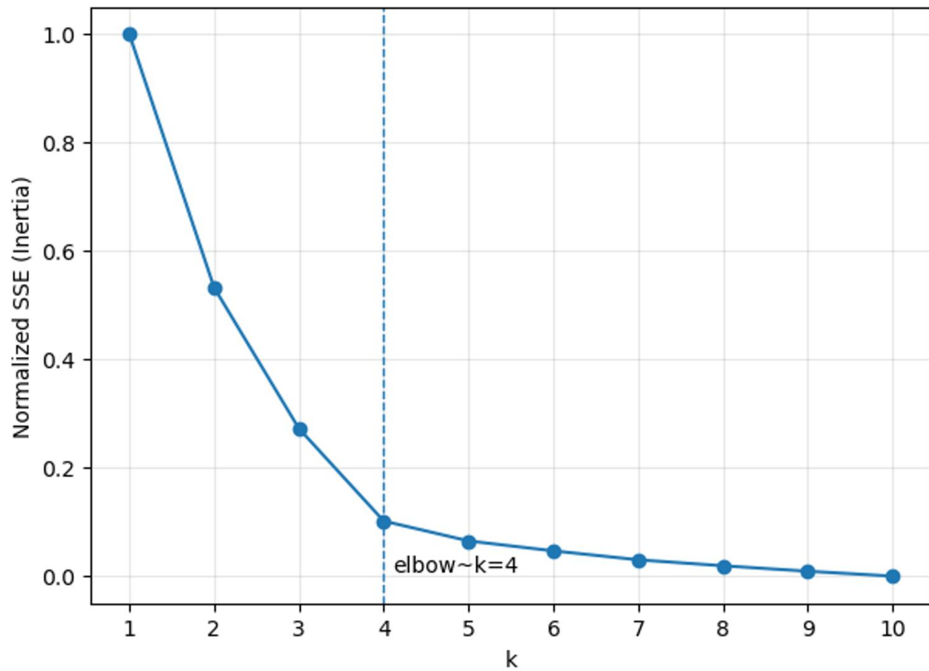
Elbow Method Curve
