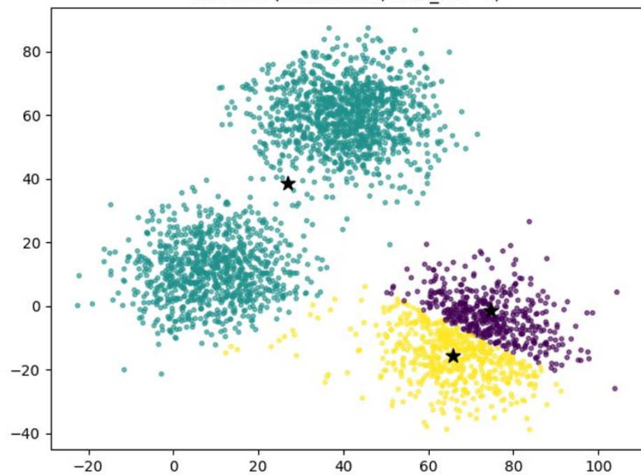
K-means (random init, max_iter=5)
