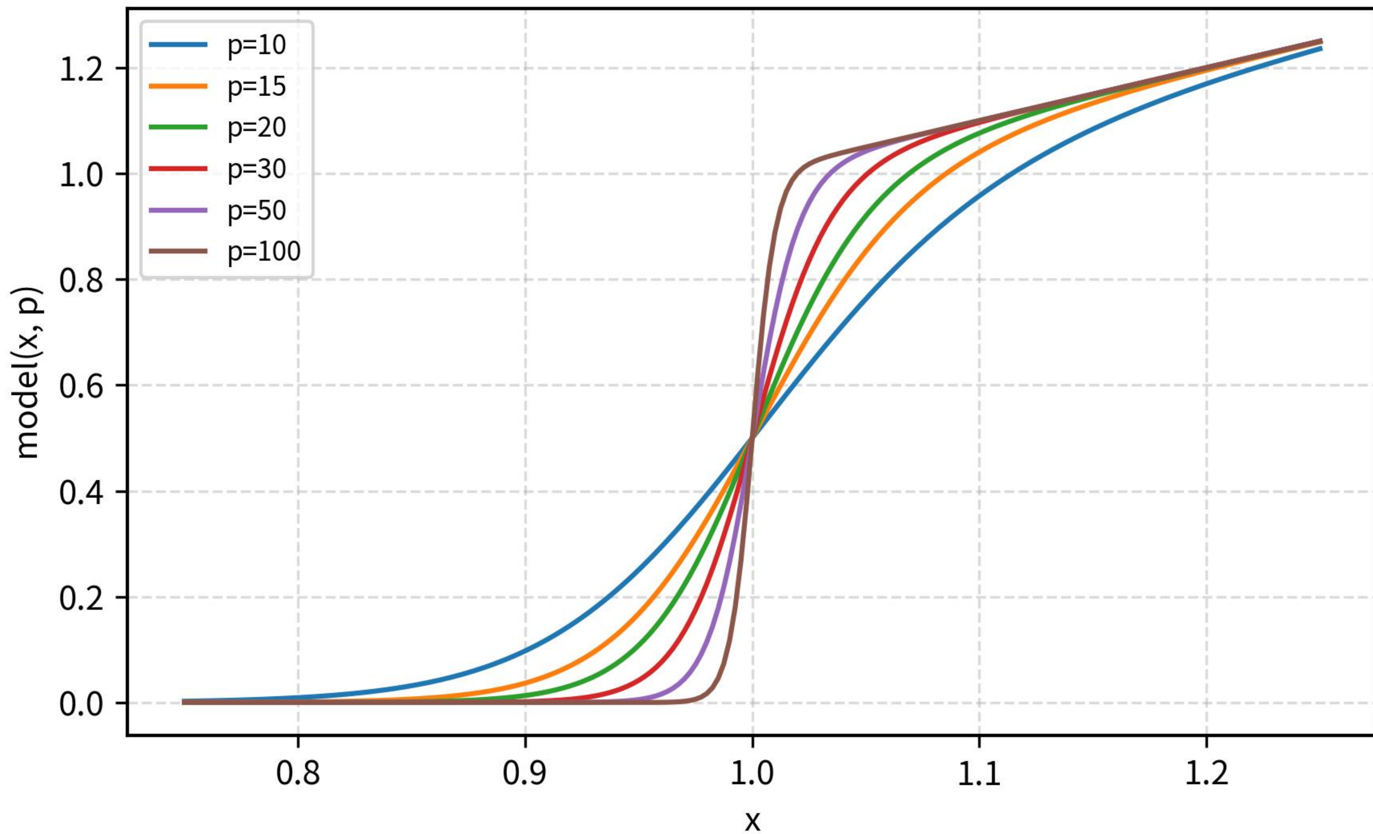
Model Curves
