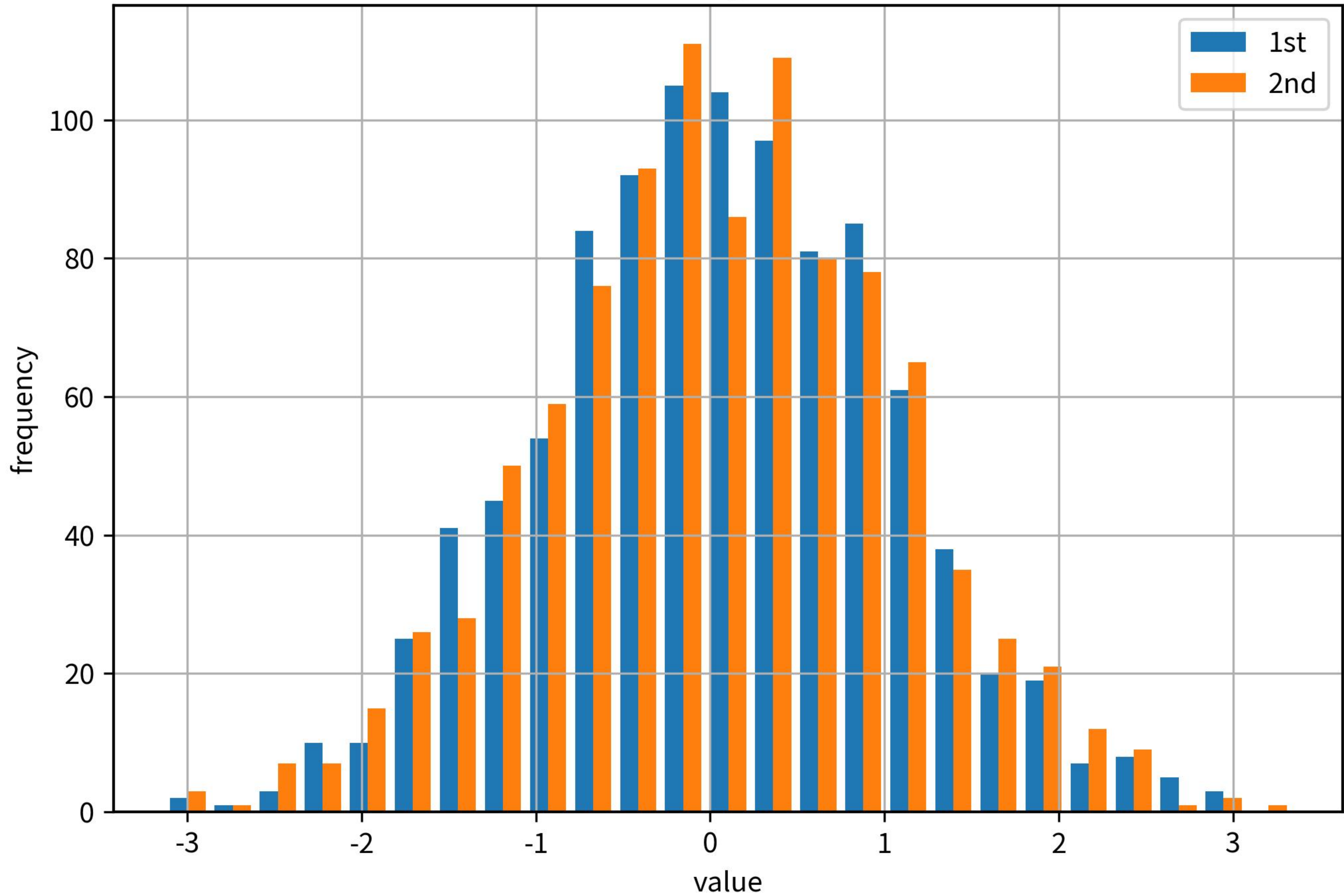
Histogram
