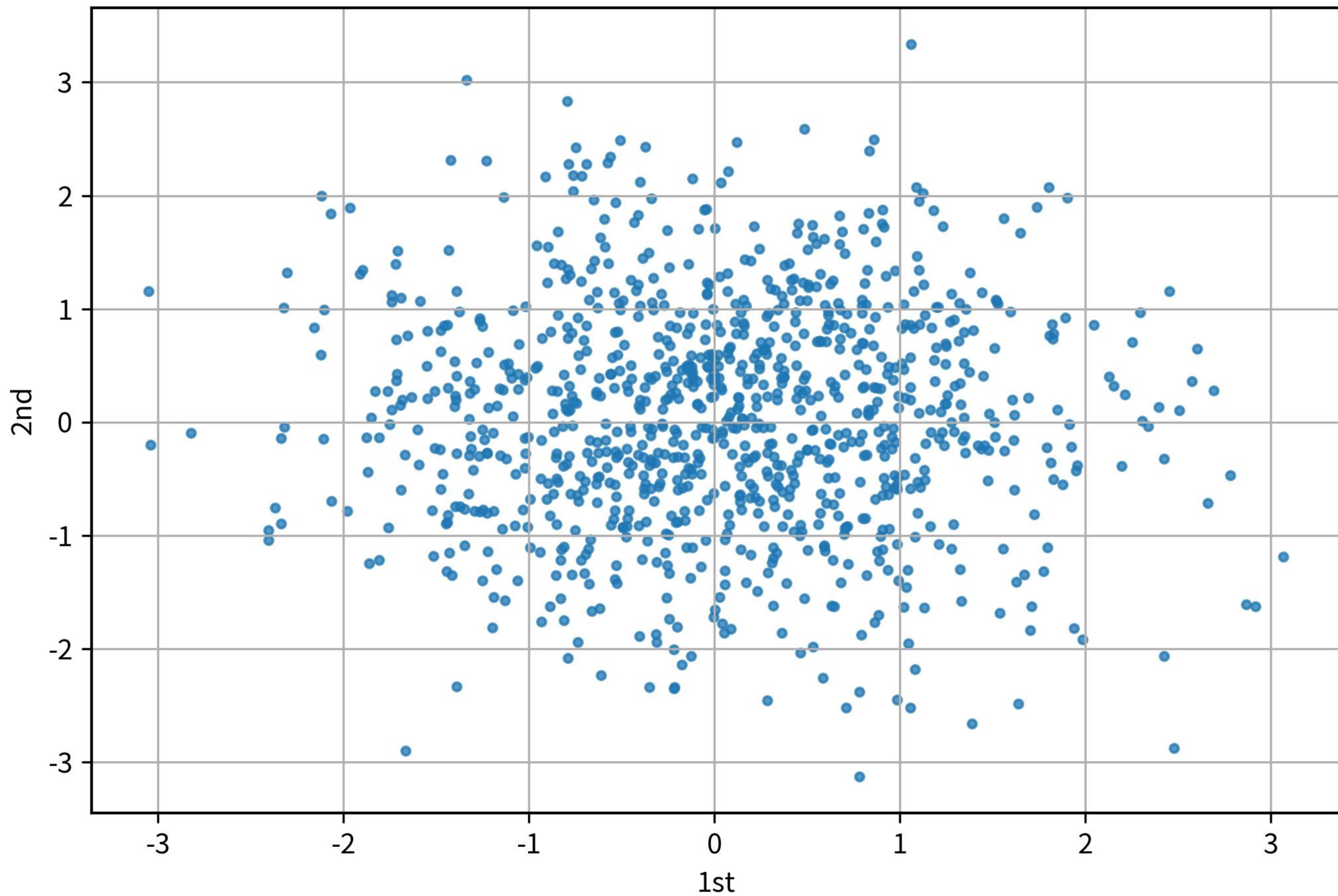
Scatter Plot
