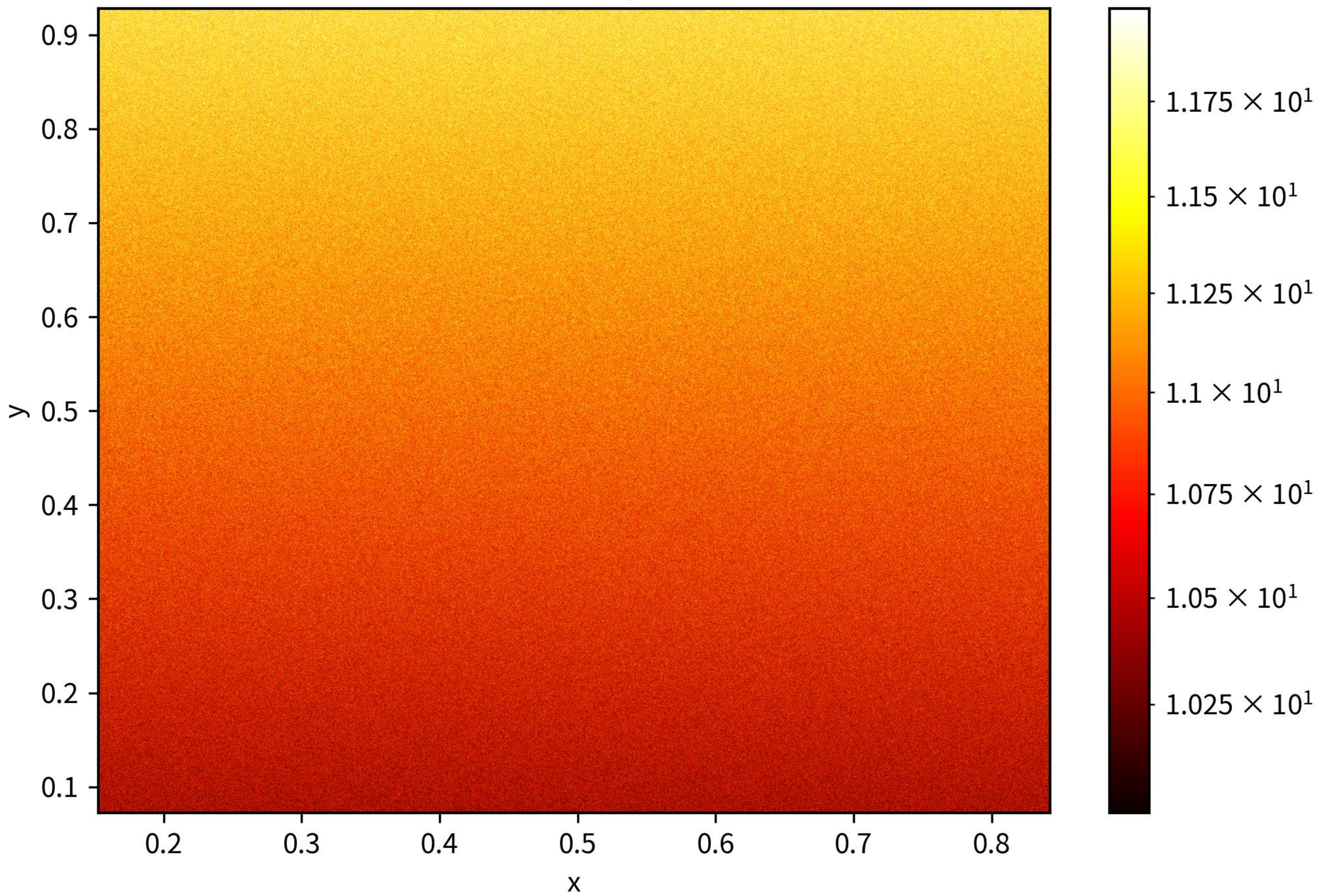
Heatmap
