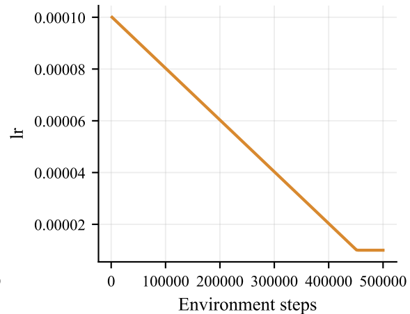
Learning rate
