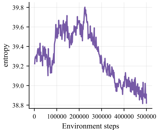
Policy entropy
