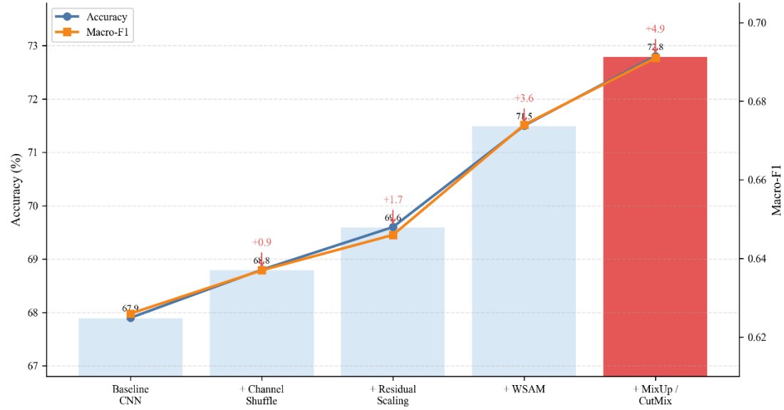
Figure 4-3. Ablation Study of EmoFormer-Lite Components
