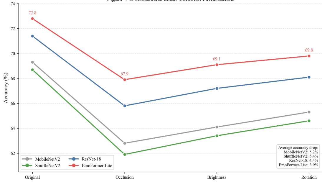
Figure 4-6. Robustness under Common Perturbations
