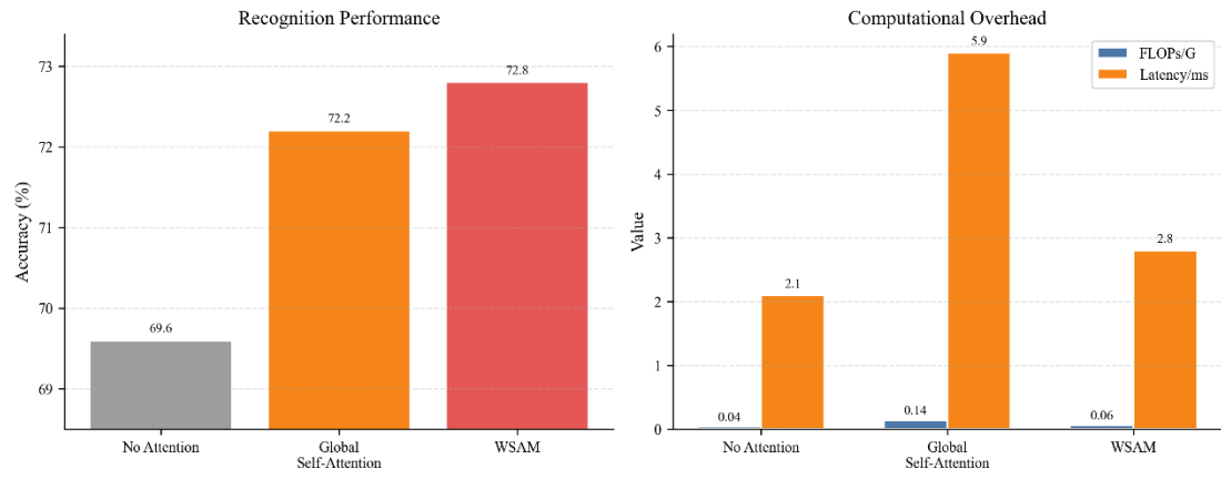
Figure 4-3. Ablation Study of EmoFormer-Lite Components
