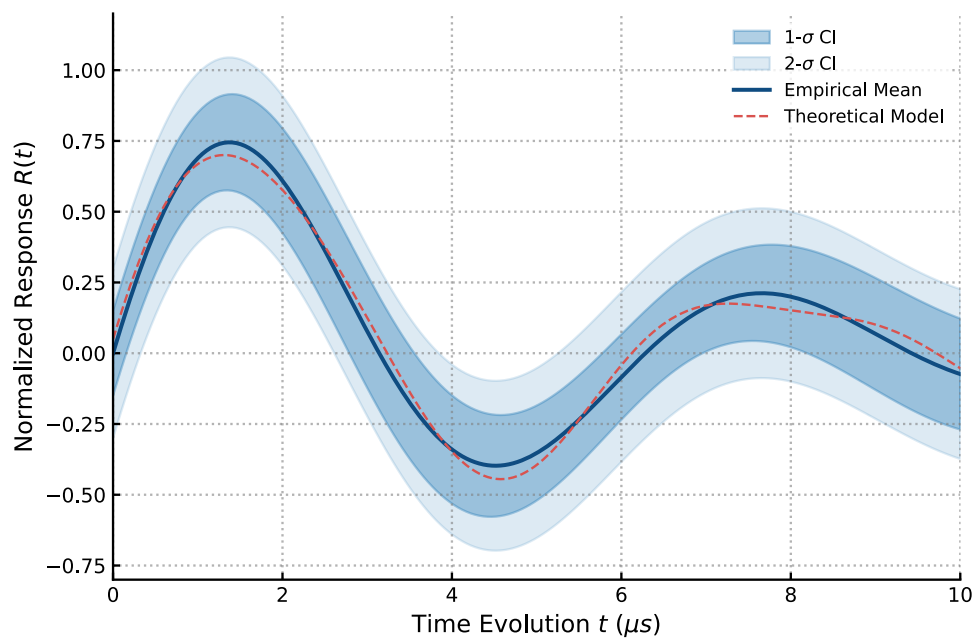
Statistical Error Analysis of Quantum Decay
