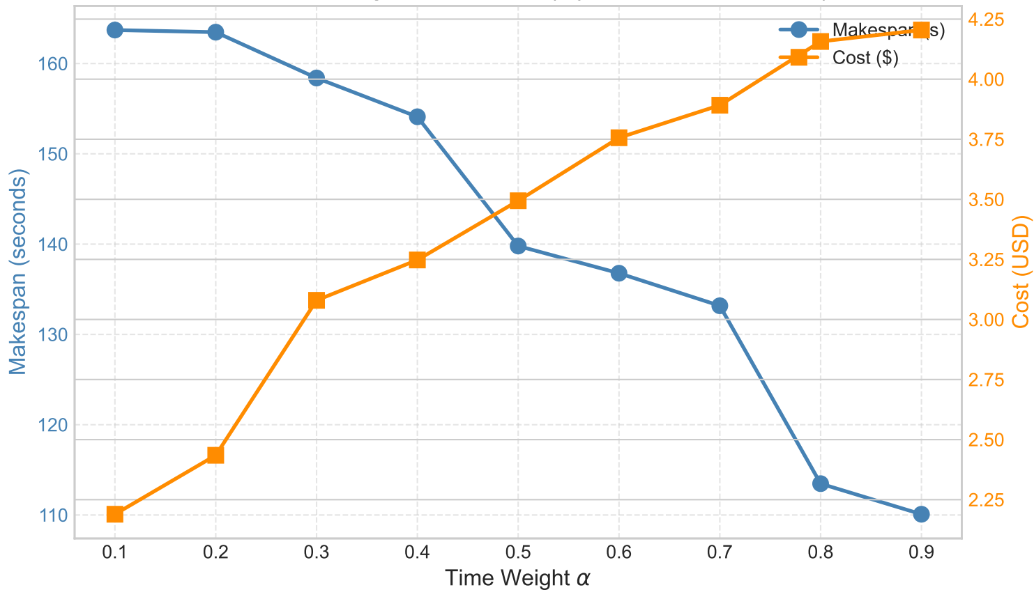
Impact of Weight Coefficient (CyberShake Workflow)
