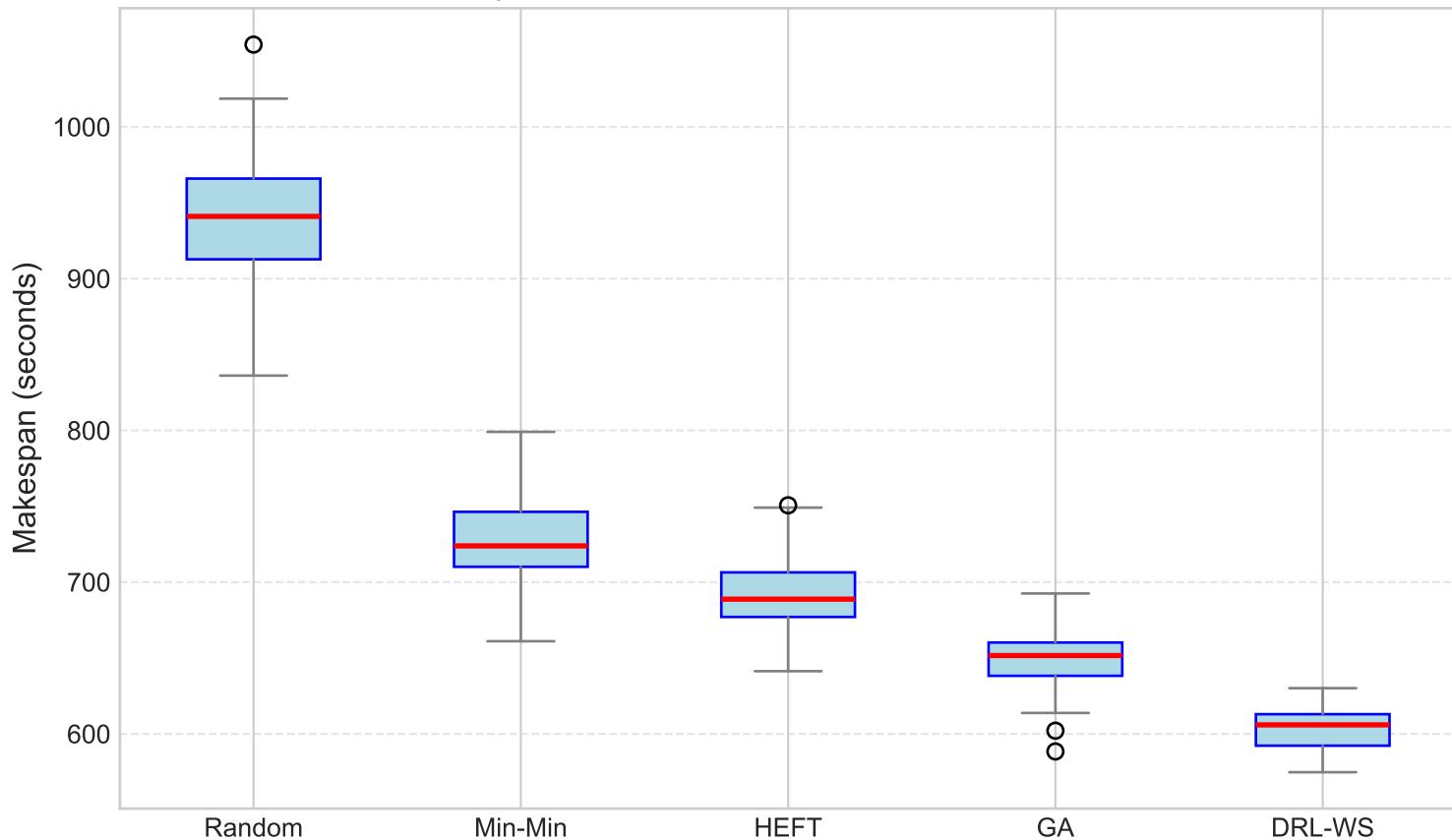
Stability of Makespan over 50 Independent Runs
