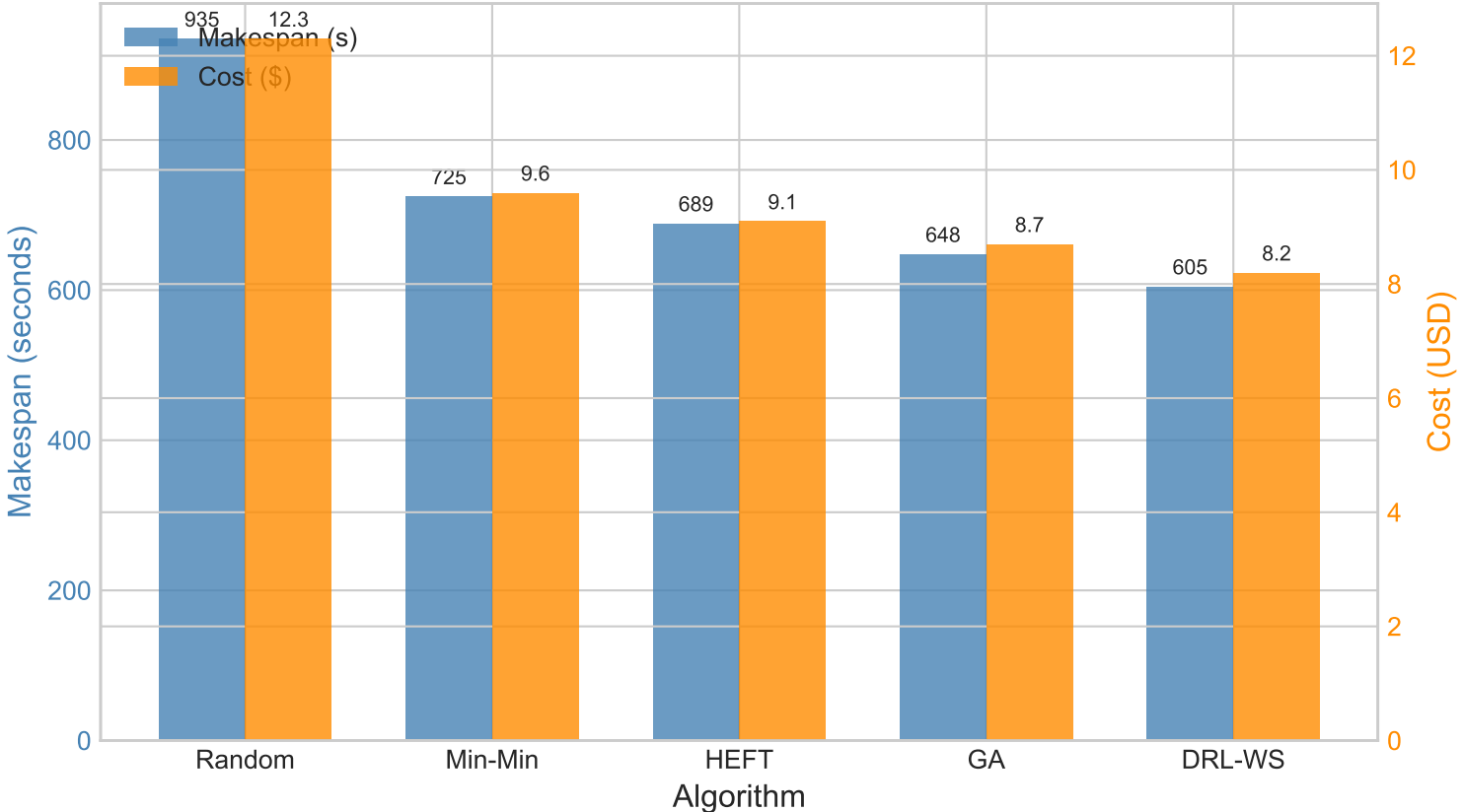
Performance Comparison on 100-task Random Workflow
