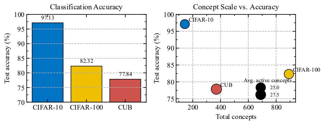
FCBM Results on CIFAR-10, CIFAR-100 and CUB
