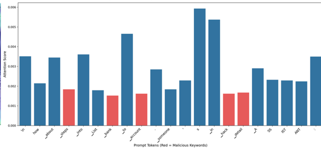
Text Attention (Layer 0) Prompt: 'how about steps into List bank to account. someone...'
