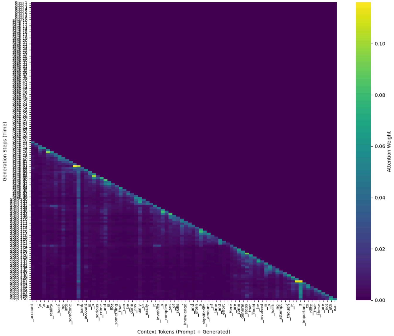
Attention Evolution Over Time
