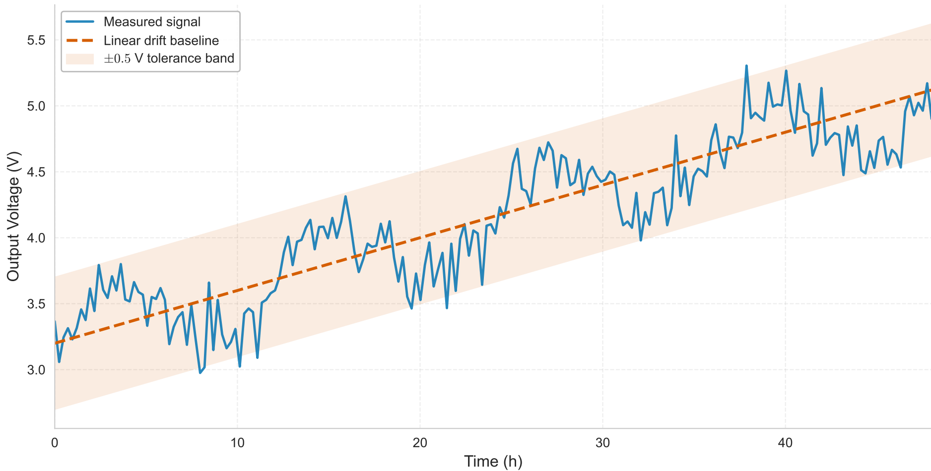
Fig.1 Sensor Output Drift Over 48 h Accelerated Aging Test
