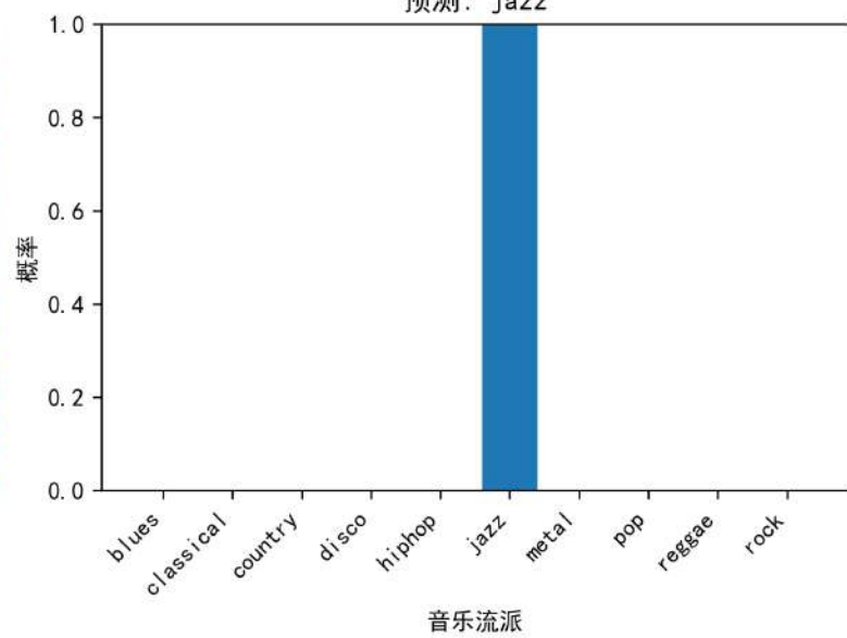
预测: jazz
