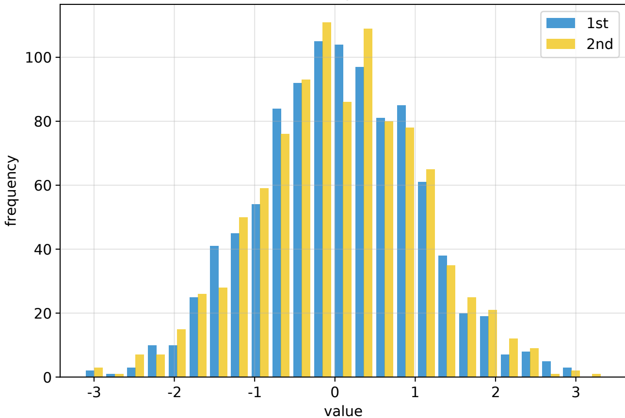
Histogram
