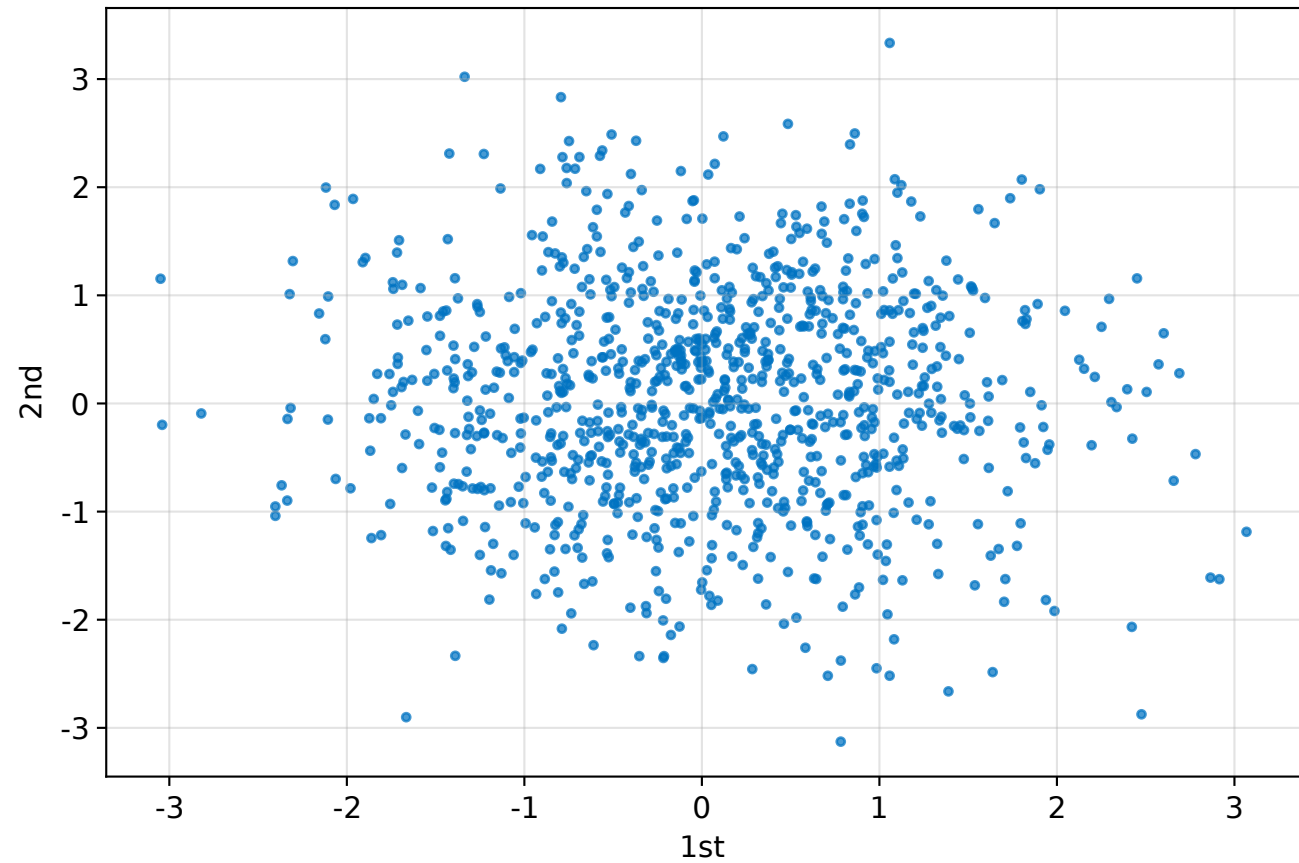
Scatter Plot
