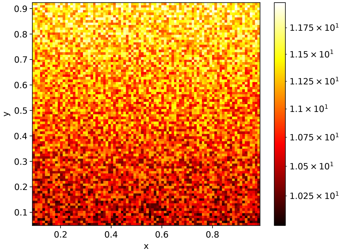
Heat Map
