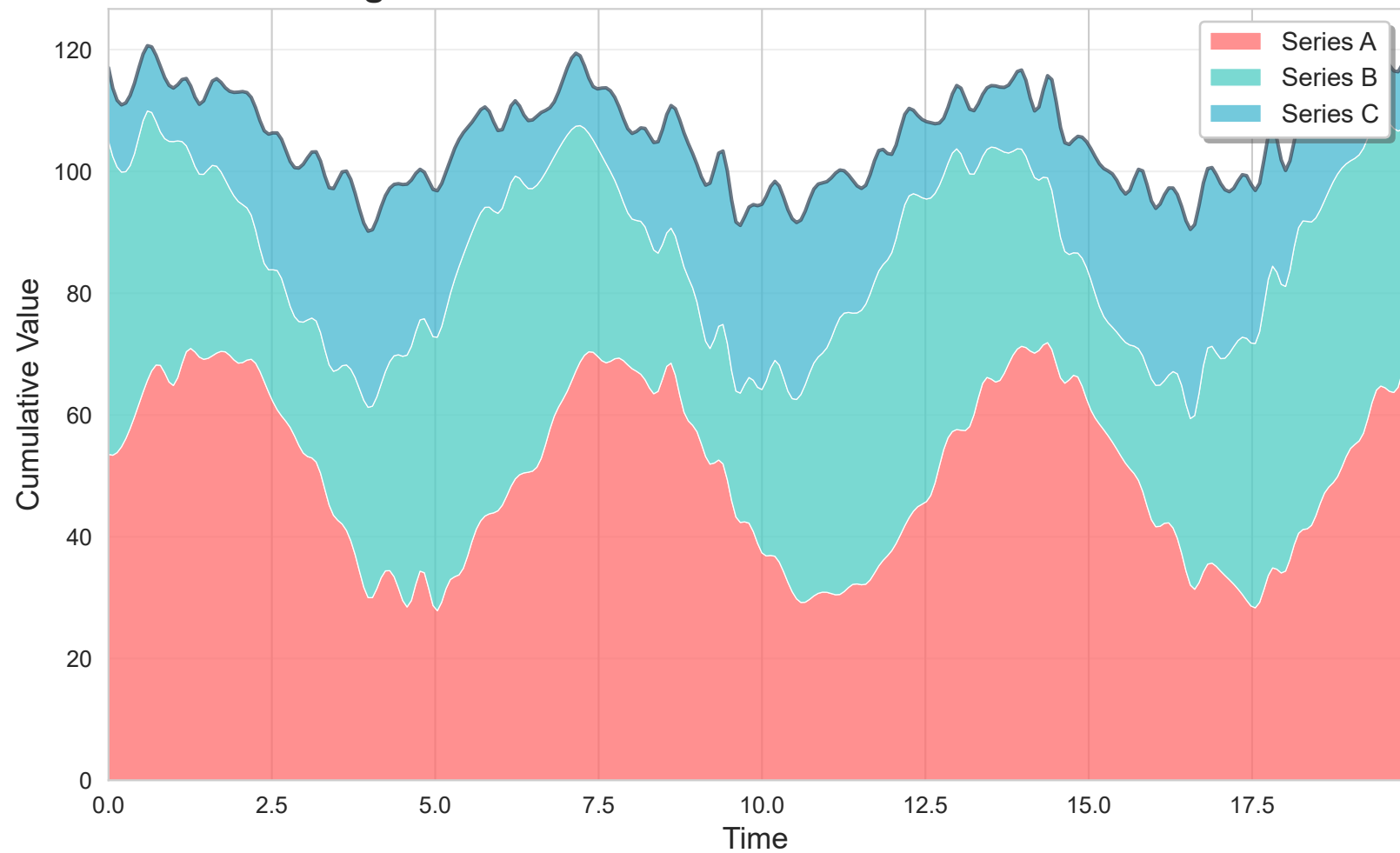
Figure 4: Stacked Area Plot with Smooth Curves
