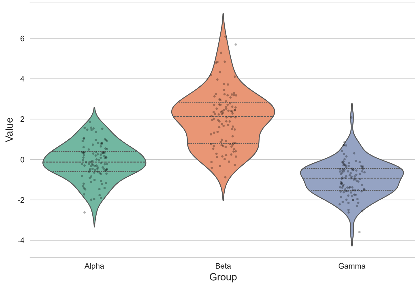
Figure 6: Grouped Violin Plots with Data Points
