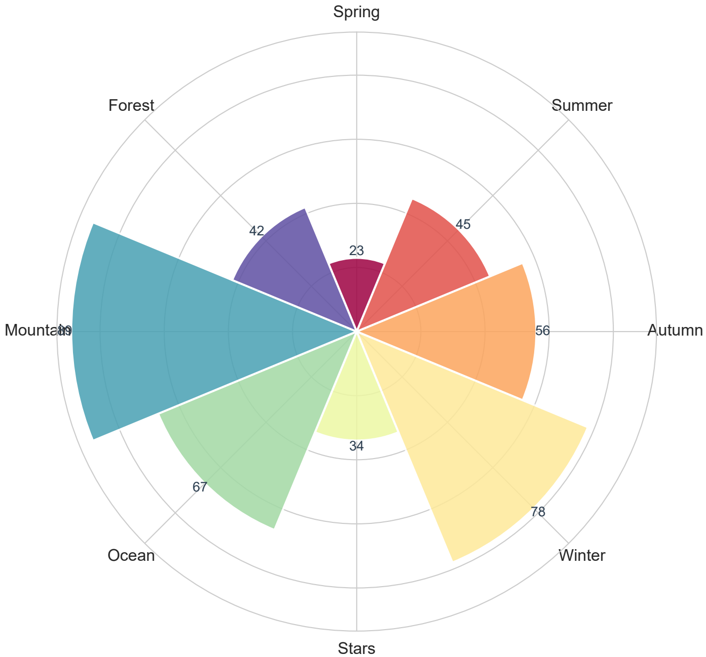
Figure 3: Nightingale Rose Chart
