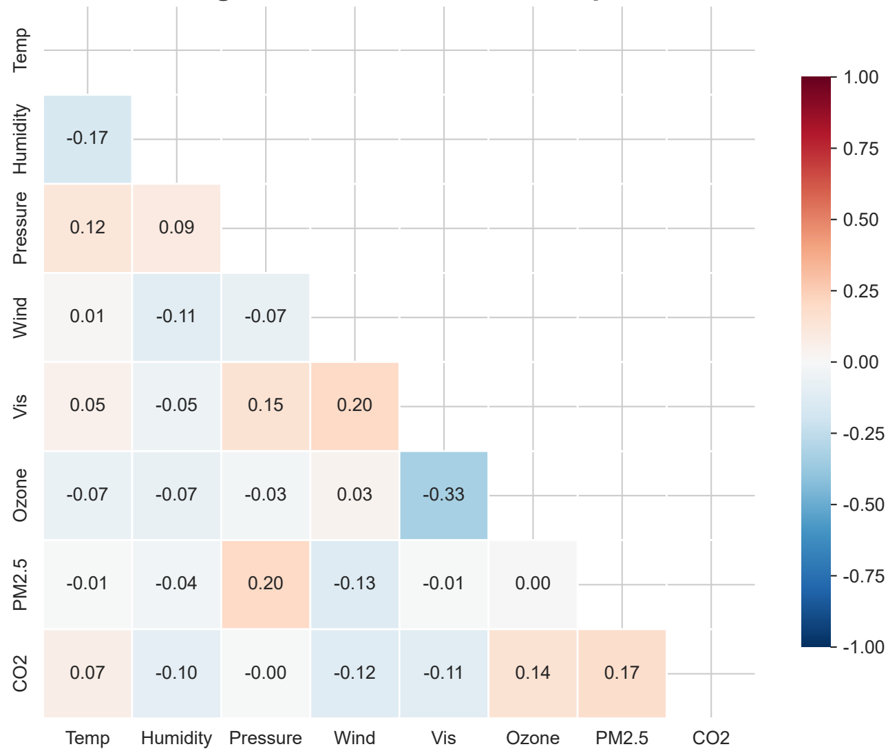
Figure 5: Correlation Heatmap
