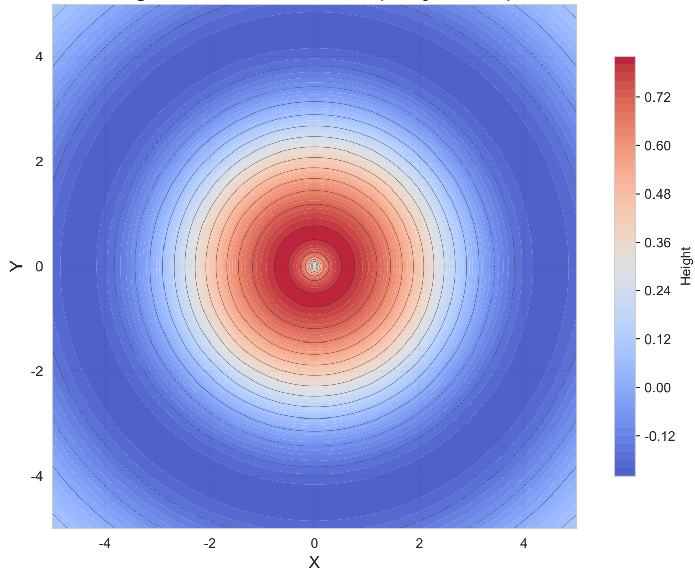
Figure 2: Filled Contours (Fully Vector)
