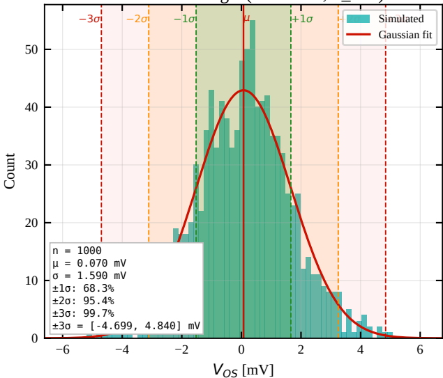
MC Offset Voltage (1000 runs, tt_mm)
