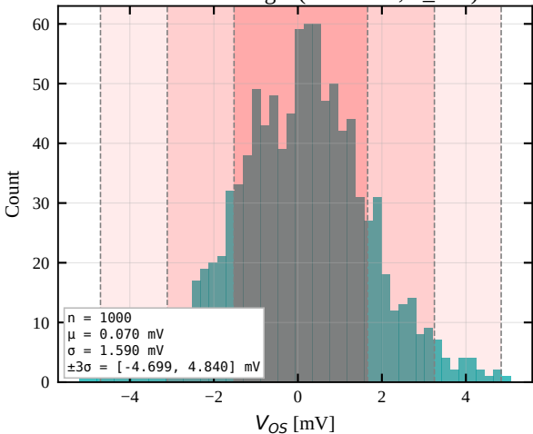
MC Offset Voltage (1000 runs, tt_mm)
