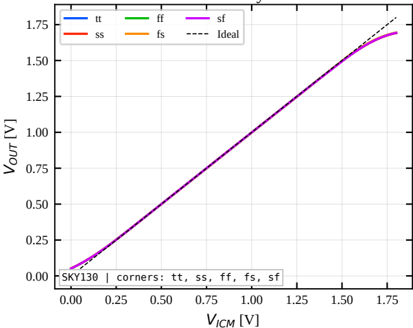
DC Transfer — Unity-Gain Buffer
