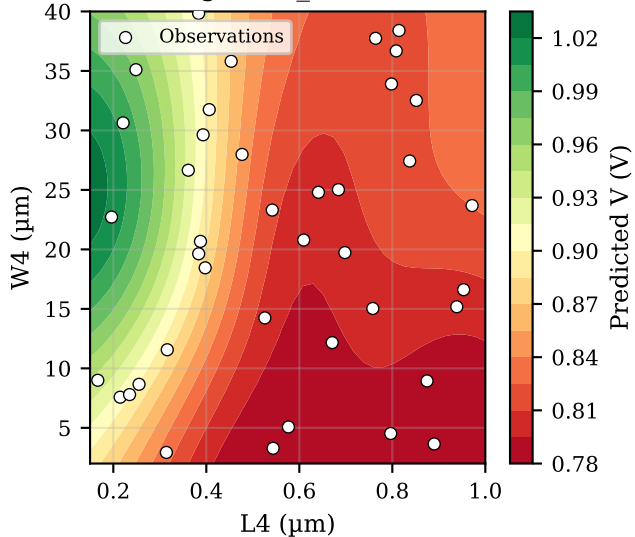
GP Surrogate: V_PL (L4 vs W4)
