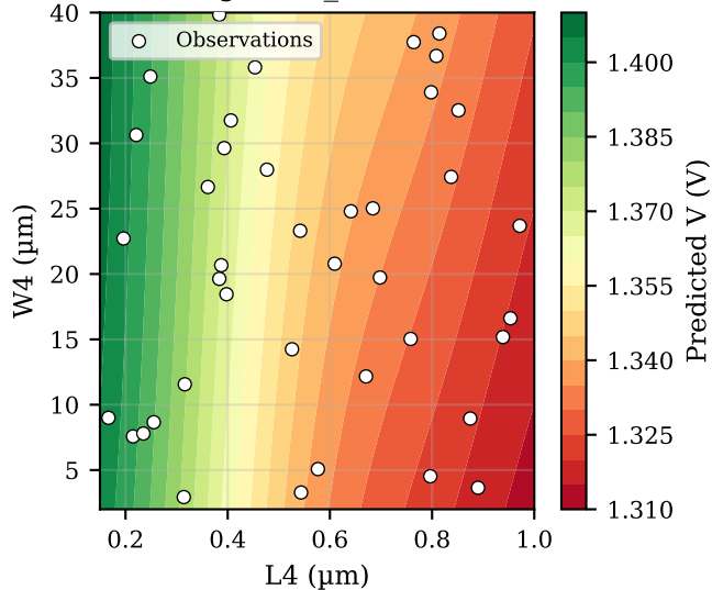
GP Surrogate: V_PH (L4 vs W4)
