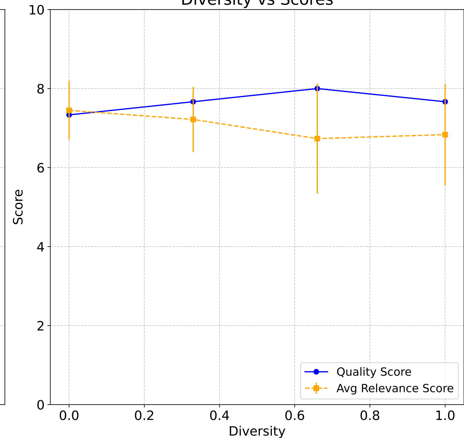
Diversity vs Scores
