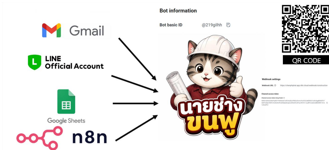
Figure 1: Overall system workflow — from site foreman (LINE) through n8n to Google Sheets and Gmail
