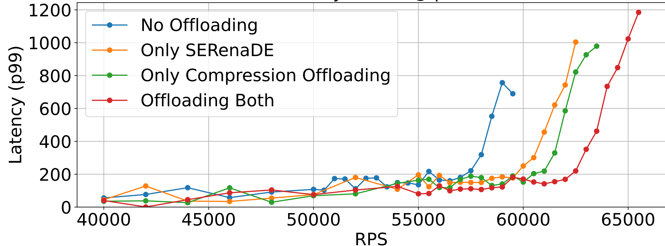
Latency vs RPS @ p99
