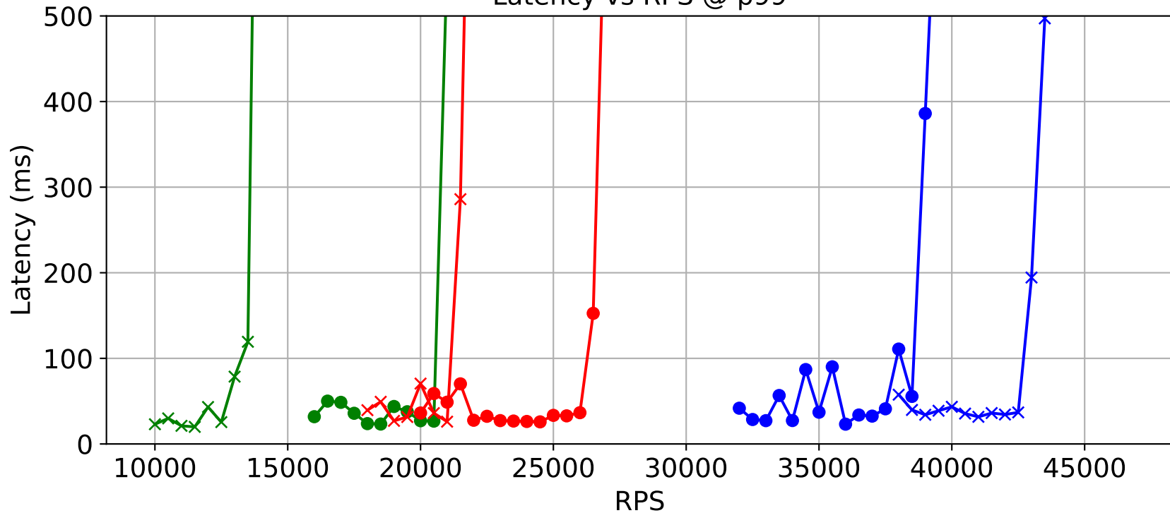
Latency vs RPS @ p99
