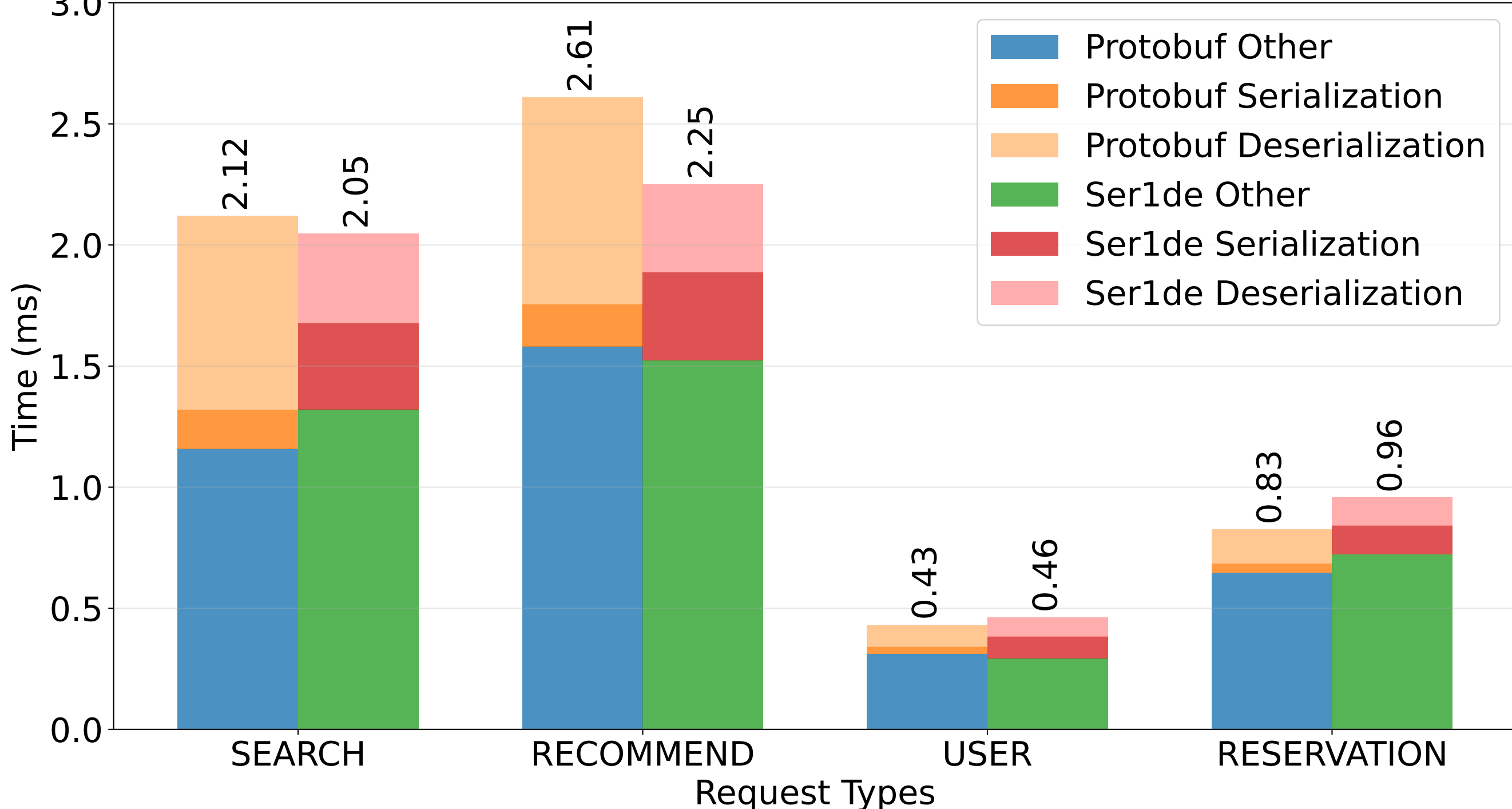
Performance Breakdown: Protobuf vs Ser1de
