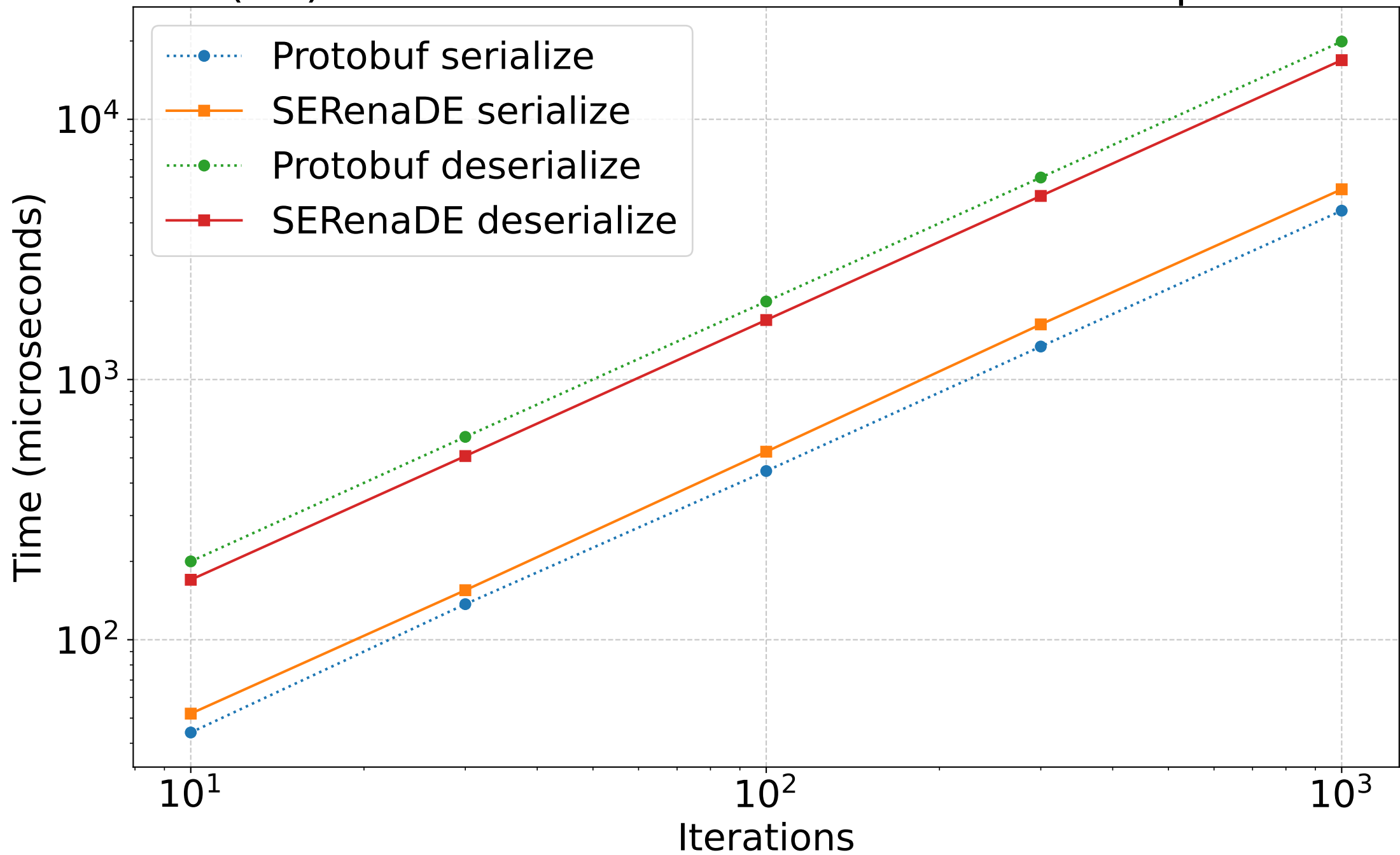
(De)Serialize Performance of Individual Requests
