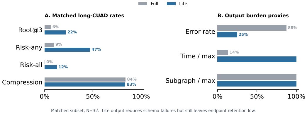
Figure 6: Naive output-burden control. Reducing the output schema helps full-SCC prompting, although it does not close the endpoint-retention gap on long CUAD components.
