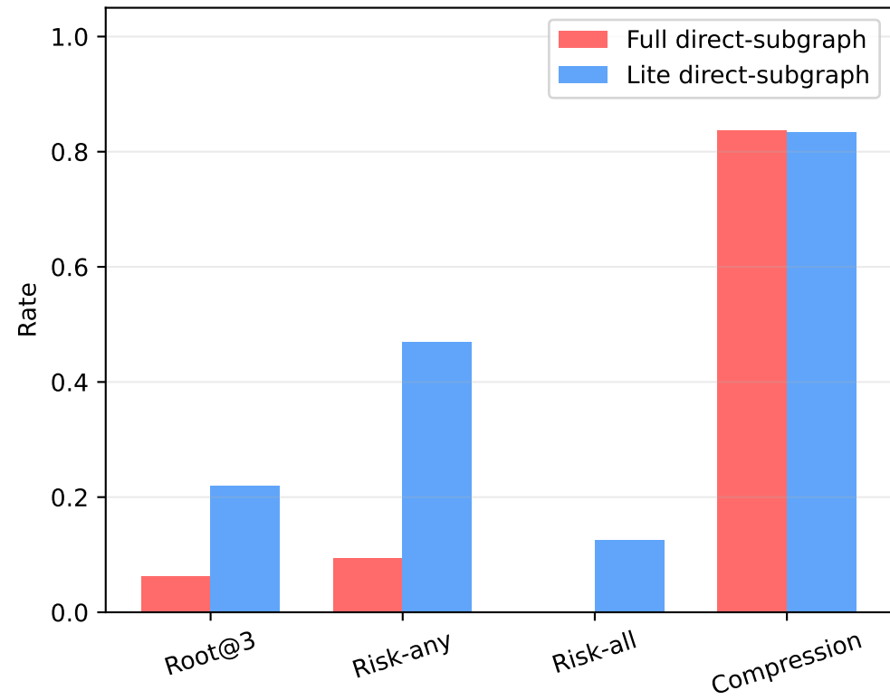
Matched metric rates
