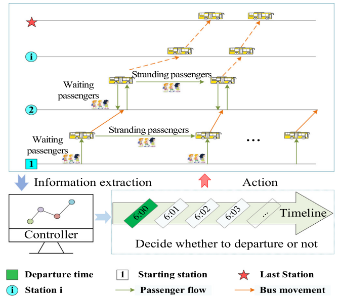
Fig. 1. The bus timetable optimization problem.
