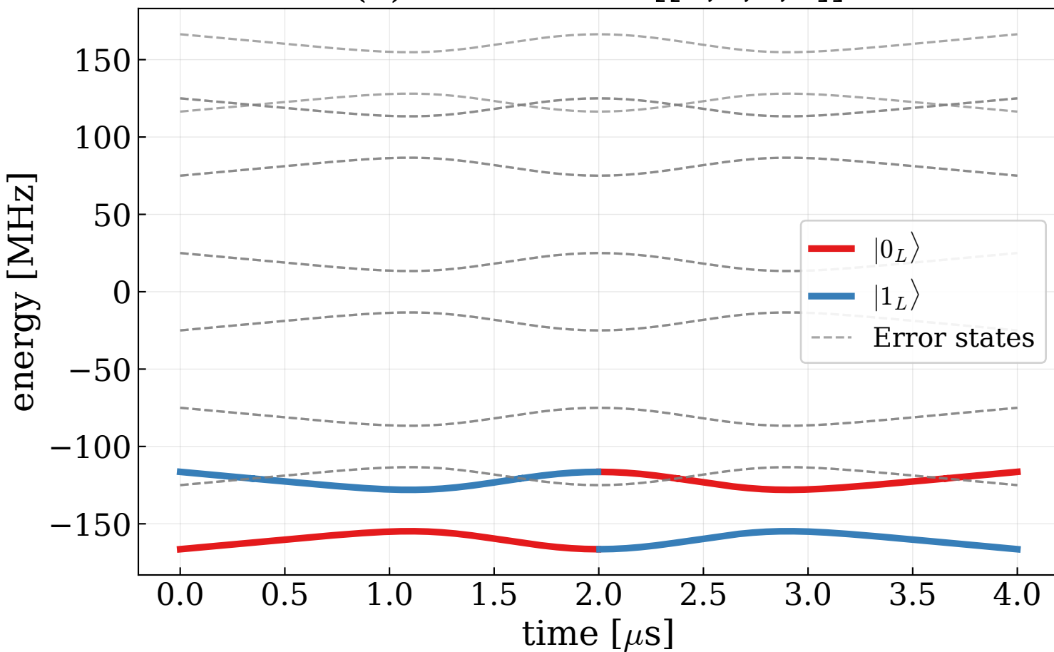
(a) Bacon-Shor [[4,1,1,2]]
