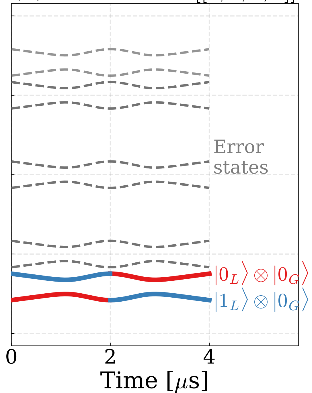
(b) Bacon-Shor [[4, 1, 1, 2]]
