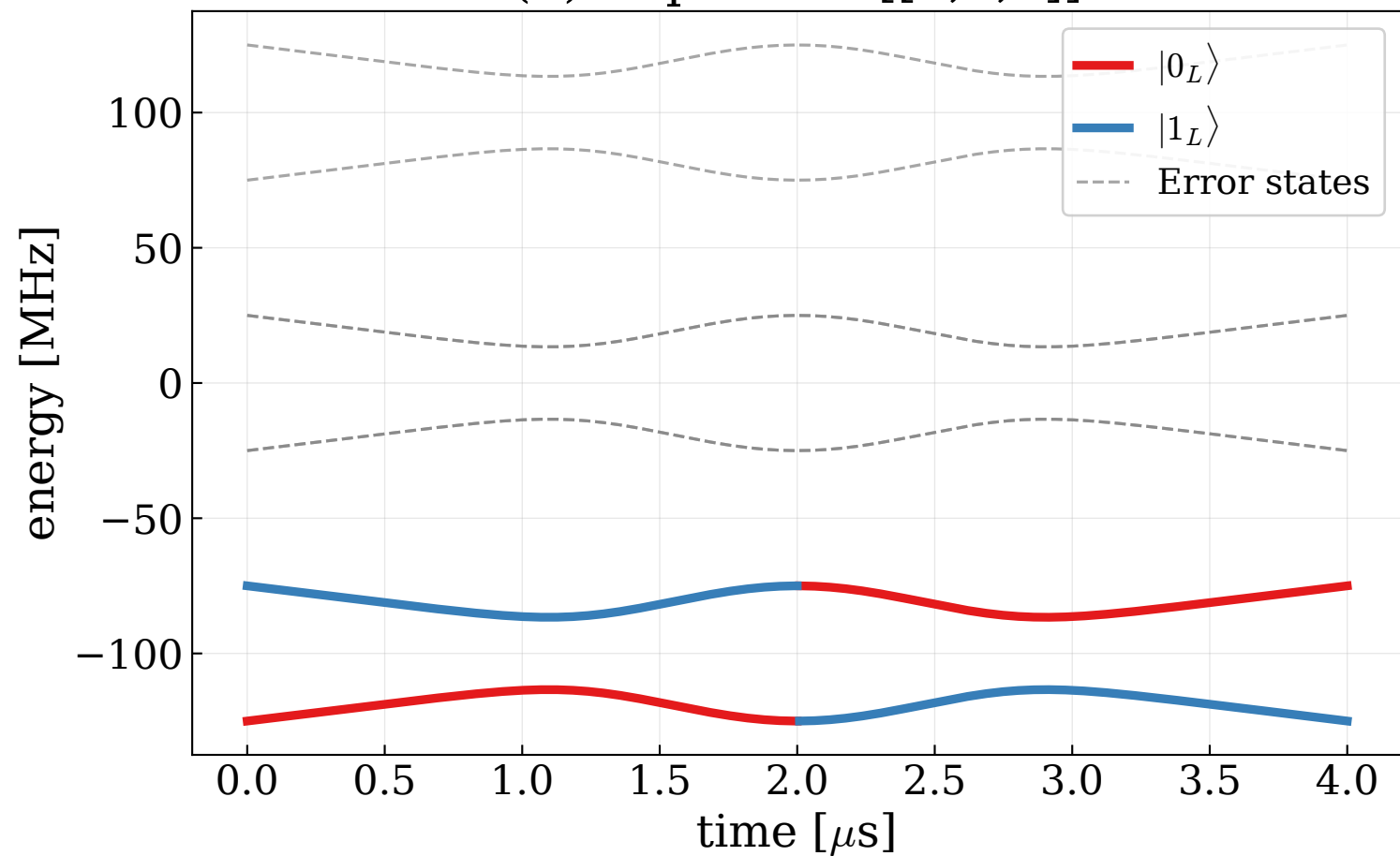
(b) Repetition [[3,1,3]]
