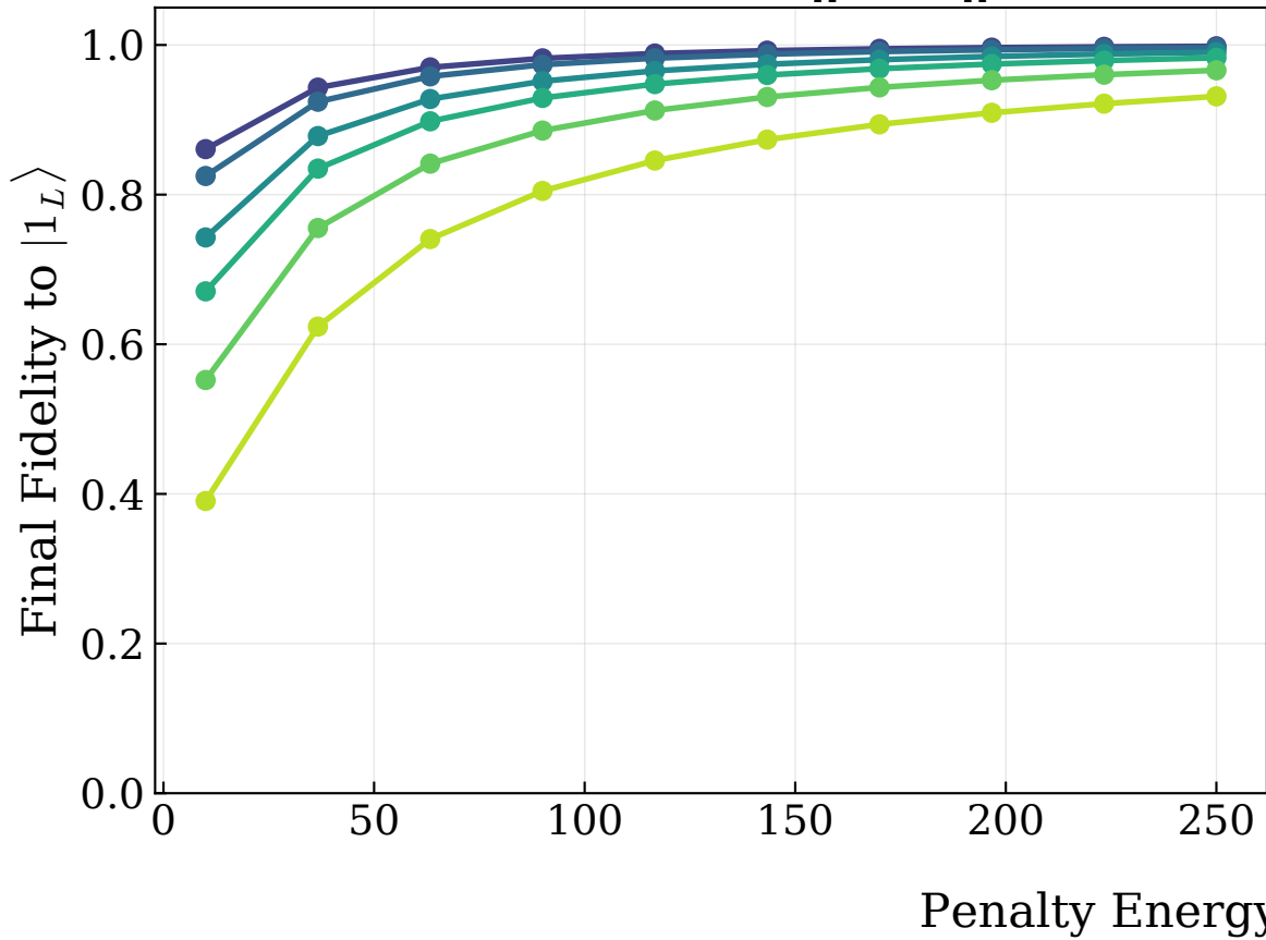
(a) Repetition [[3, 1, 3]]
