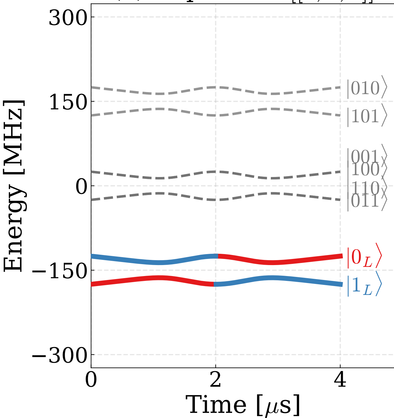
(a) Repetition [[3, 1, 3]]
