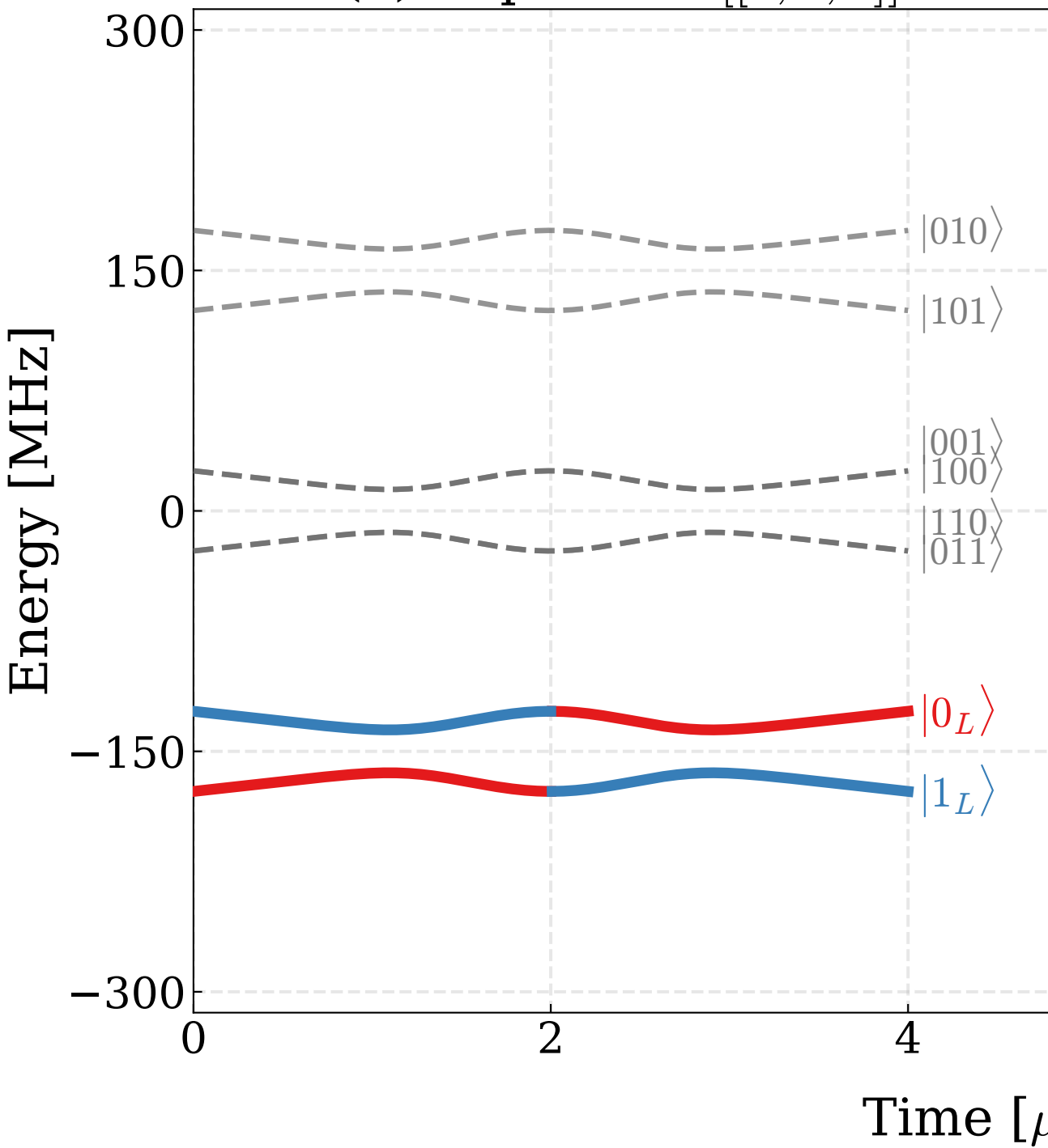
(a) Repetition [[3, 1, 3]]
