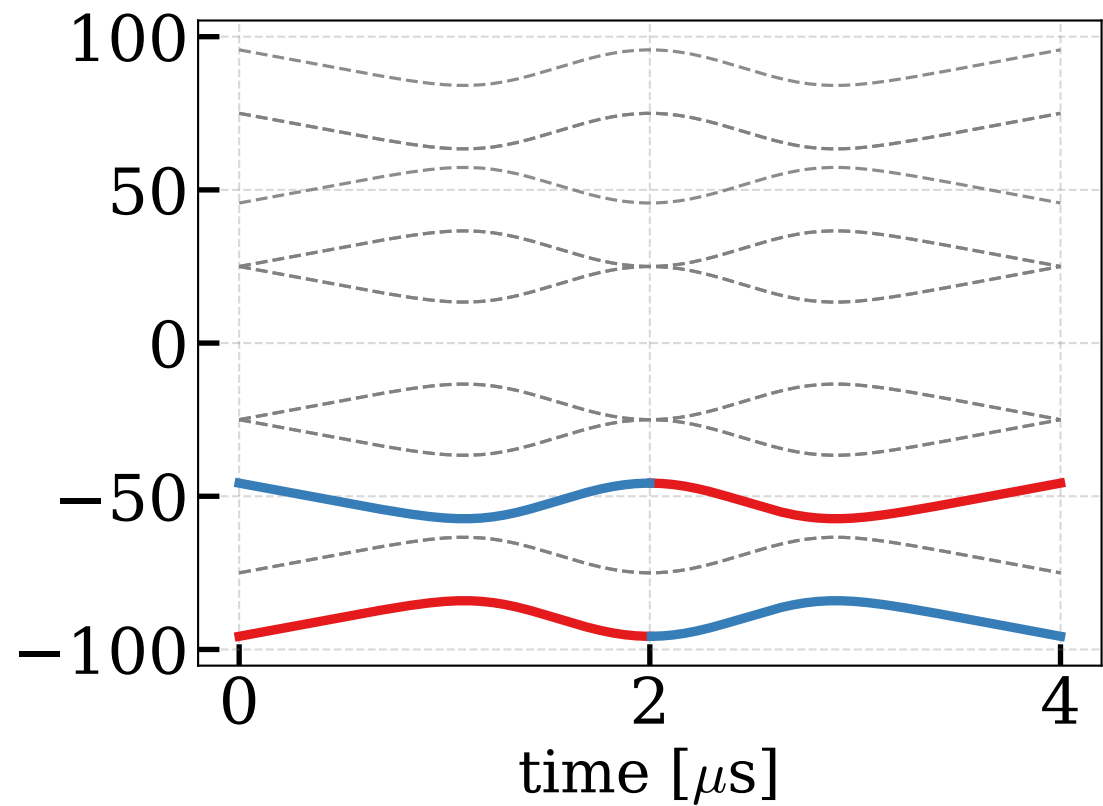
Bacon-Shor [[4,1,1,2]] : Energy spectrum with gauge penalization E_p = 0 [MHz] E_p = 25 [MHz] E_p = 100 [MHz]
