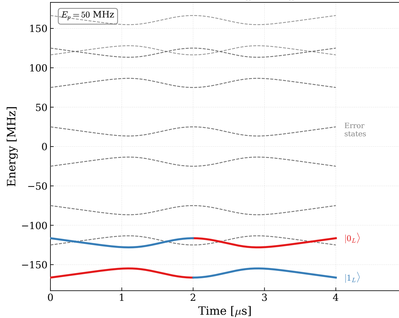
(b) Bacon-Shor [[4, 1, 1, 2]]
