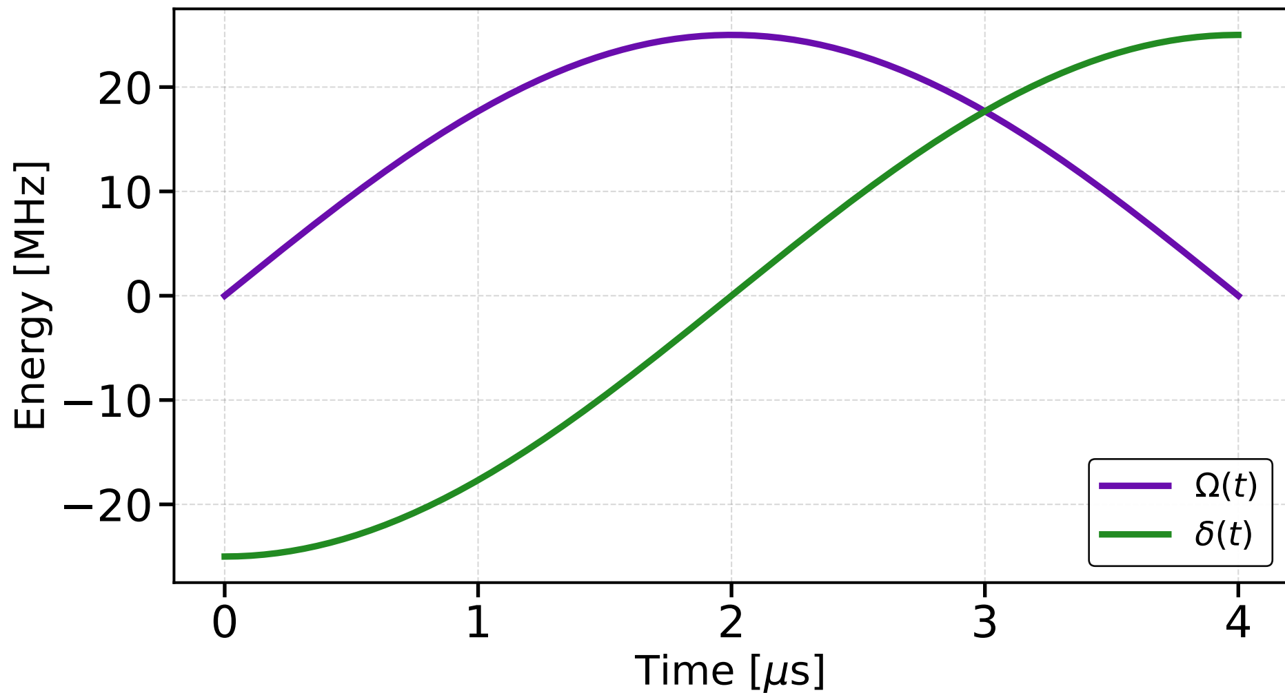
Sinusoidal RAP Pulse Profiles (IBM Platform)
