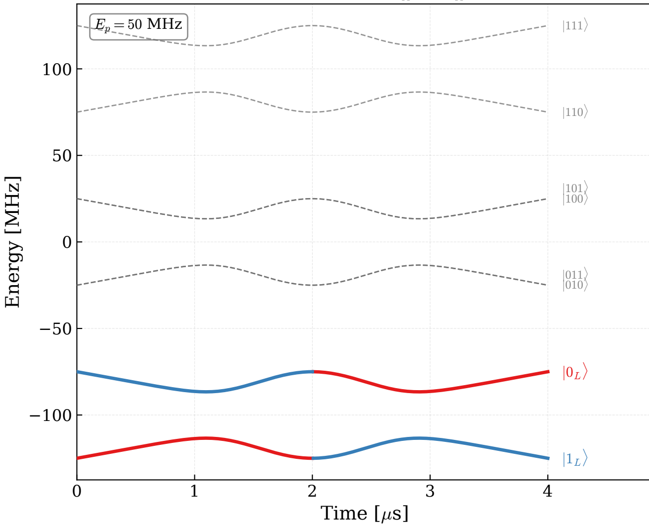
(a) Repetition [[3, 1, 3]]
