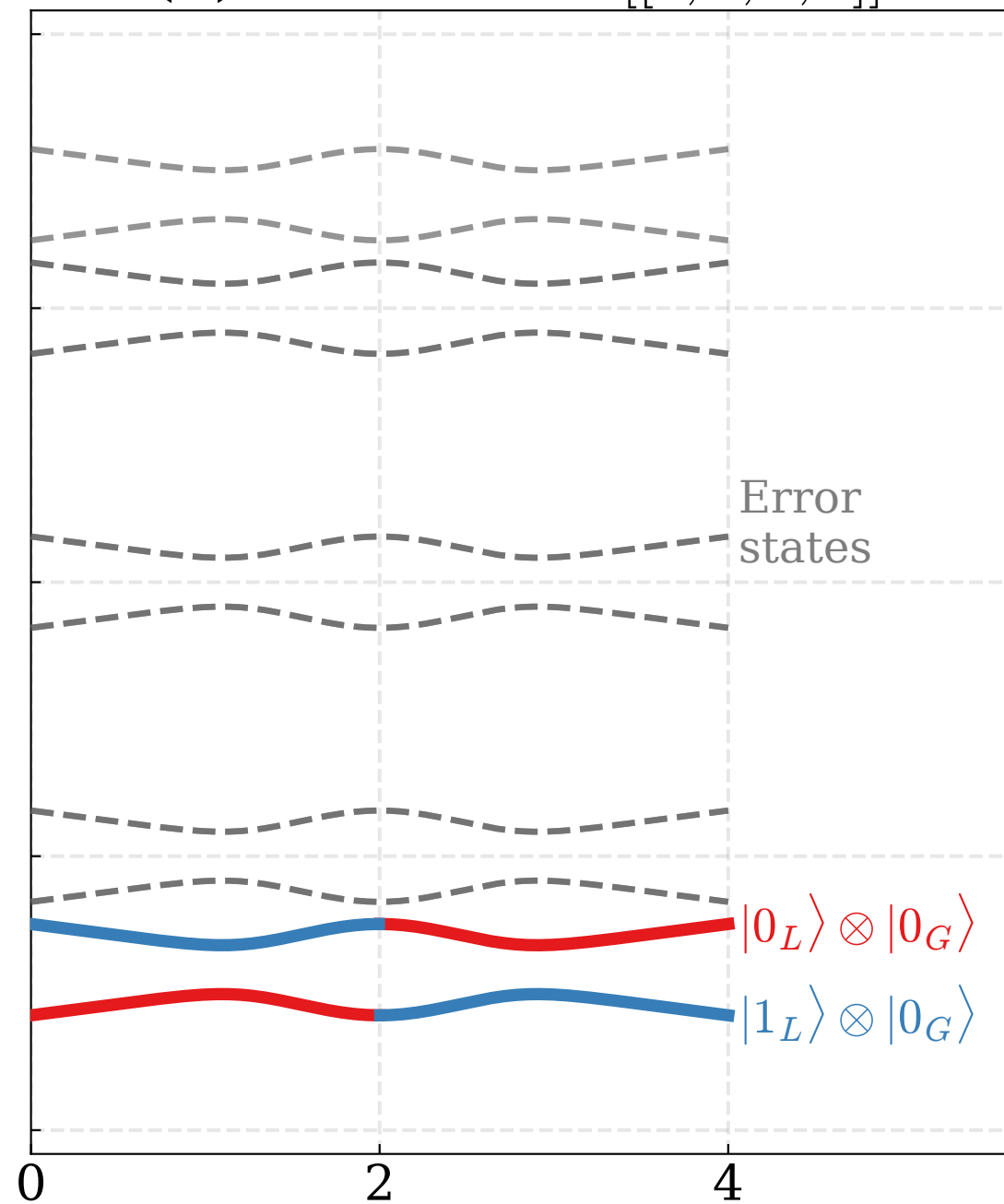
(b) Bacon-Shor [[4, 1, 1, 2]]
