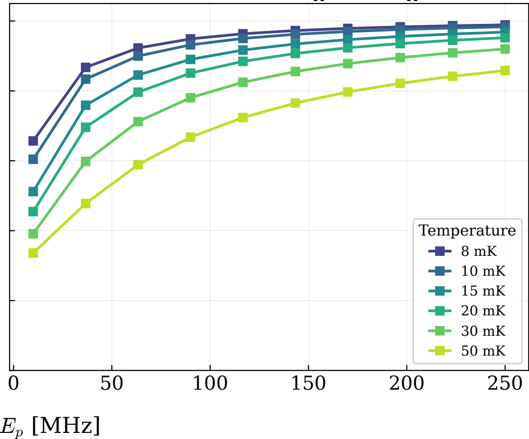
(b) Bacon-Shor [[4, 1, 1, 2]]
