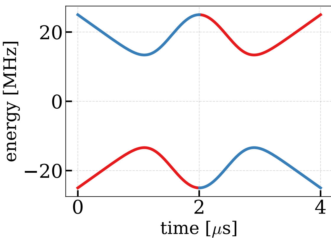
Bacon-Shor [[4,1,1,2]] : Energy spectrum with gauge penalization E_p = 0 [MHz] E_p = 25 [MHz] E_p = 100 [MHz]
