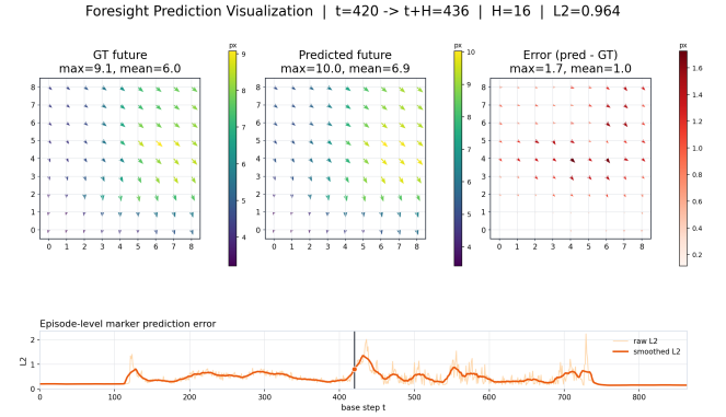
Fig. 5. Predicted versus observed tactile consequence. Example board-wiping visualization comparing predicted marker displacement fields with ground-truth future observations at the long horizon.
