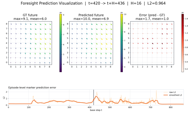
Fig. 5. Predicted versus observed tactile consequence. Example board-wiping visualization comparing predicted marker displacement fields with ground-truth future observations at the long horizon.
