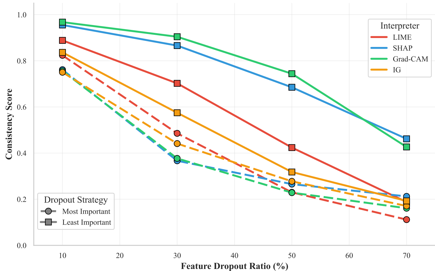
Consistency Scores Under Different Feature Dropout Strategies
