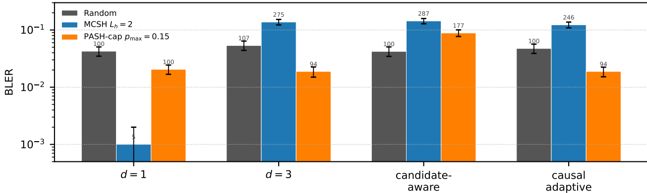
Coded BLER (mixture-LLR, adaptive frame count, bootstrap 95% CI)
