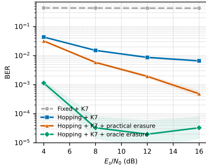
(c) One-symbol-delayed reactive jammer
