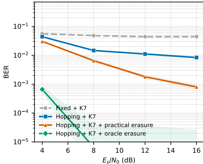
(b) Sweep jammer: matched coding
