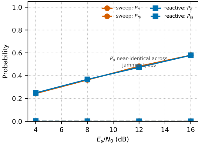
(b) Practical detector: P_d (solid), P_{fa} (dashed)
